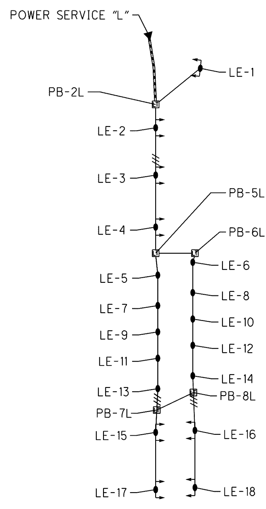
CIRCUIT E POWER SERVICE "L"
