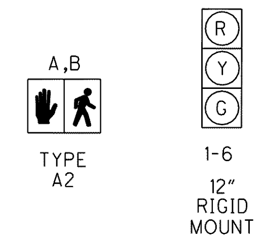
SIGNAL INDICATIONS
