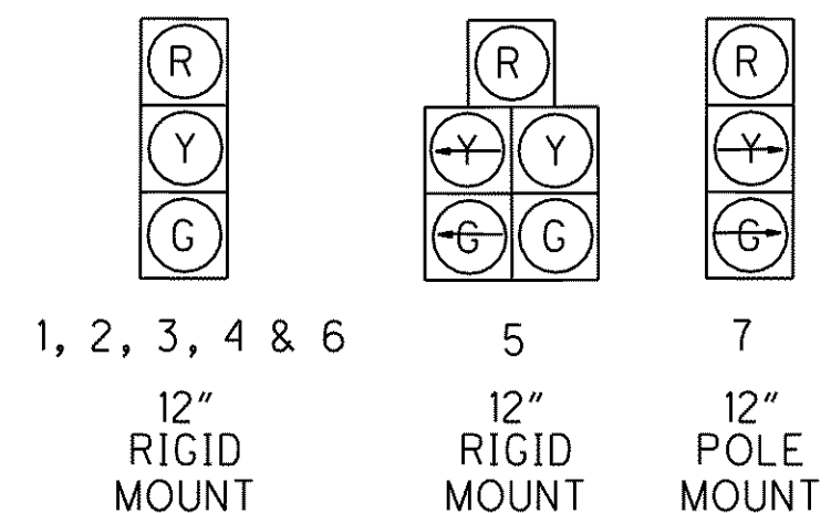
SIGNAL INDICATIONS
