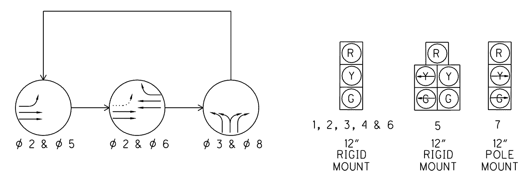
PHASING DIAGRAM
