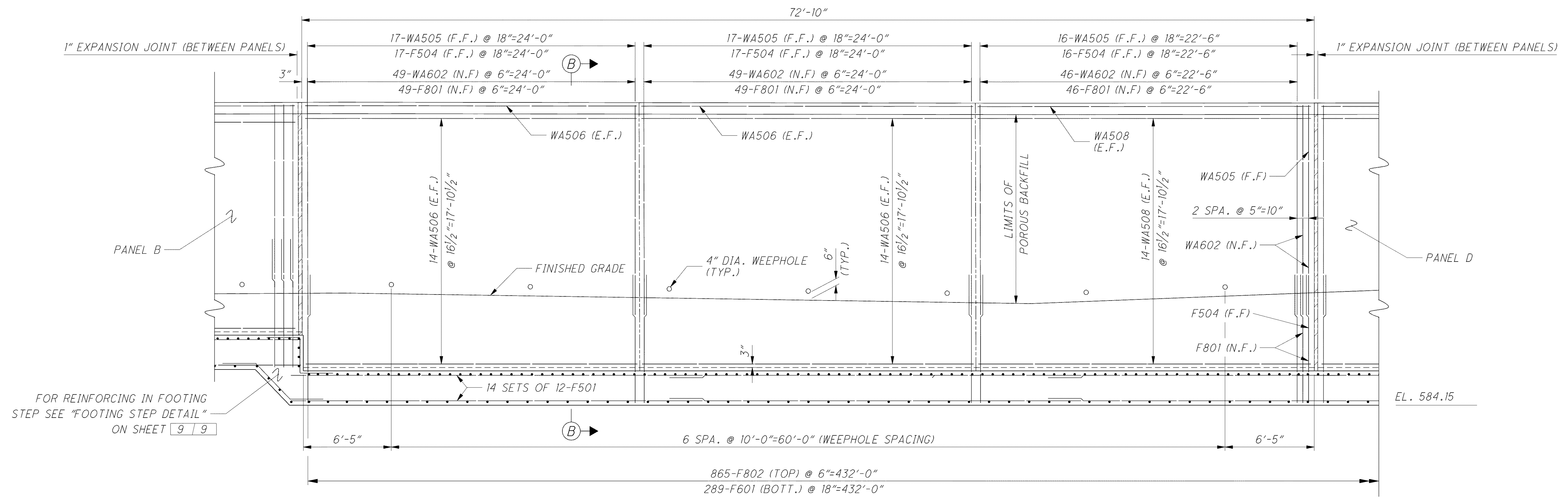
PANEL C (RECESSED PANEL NOT SHOWN FOR CLARITY)
