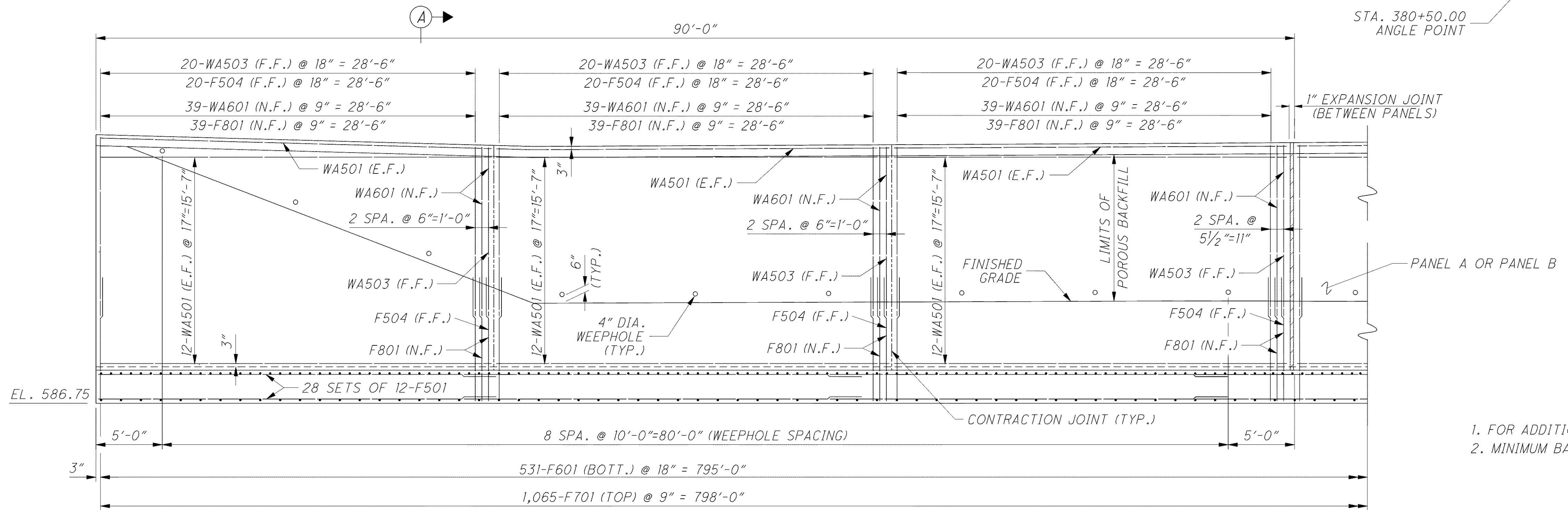
PANEL A (RECESSED PANEL NOT SHOWN FOR CLARITY)
