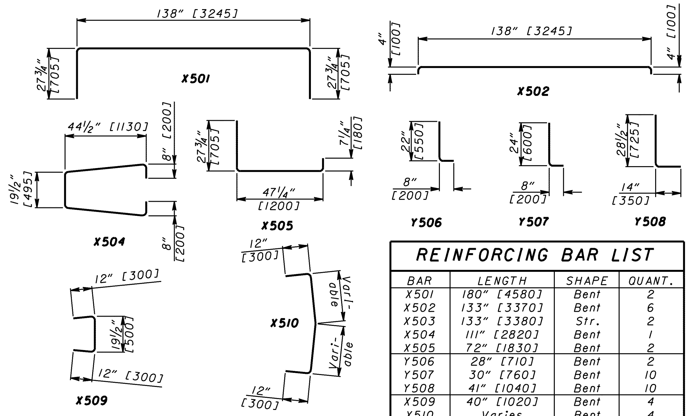
BENDING DIAGRAMS
