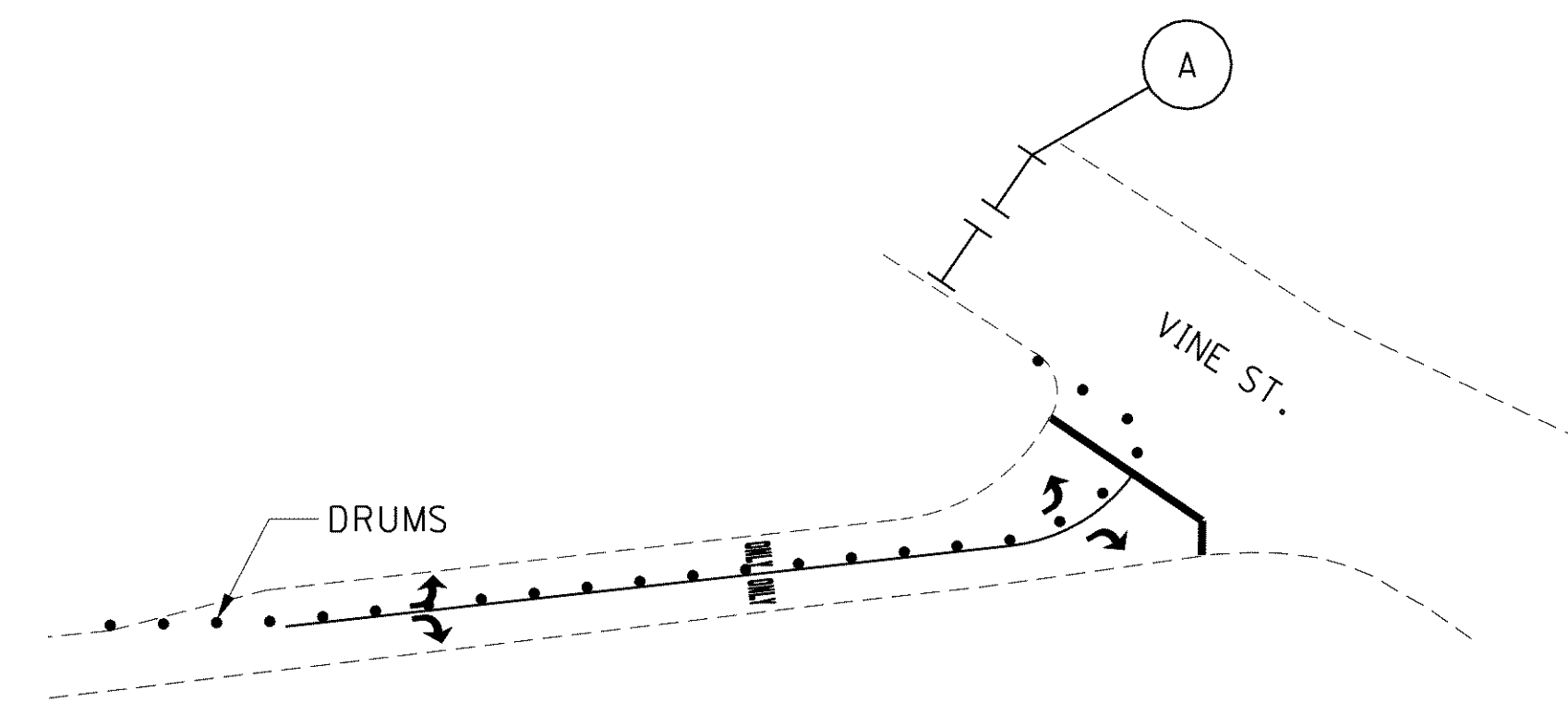
DETAIL 'A' WB RAMP LEFT TURN LANE CLOSURE
