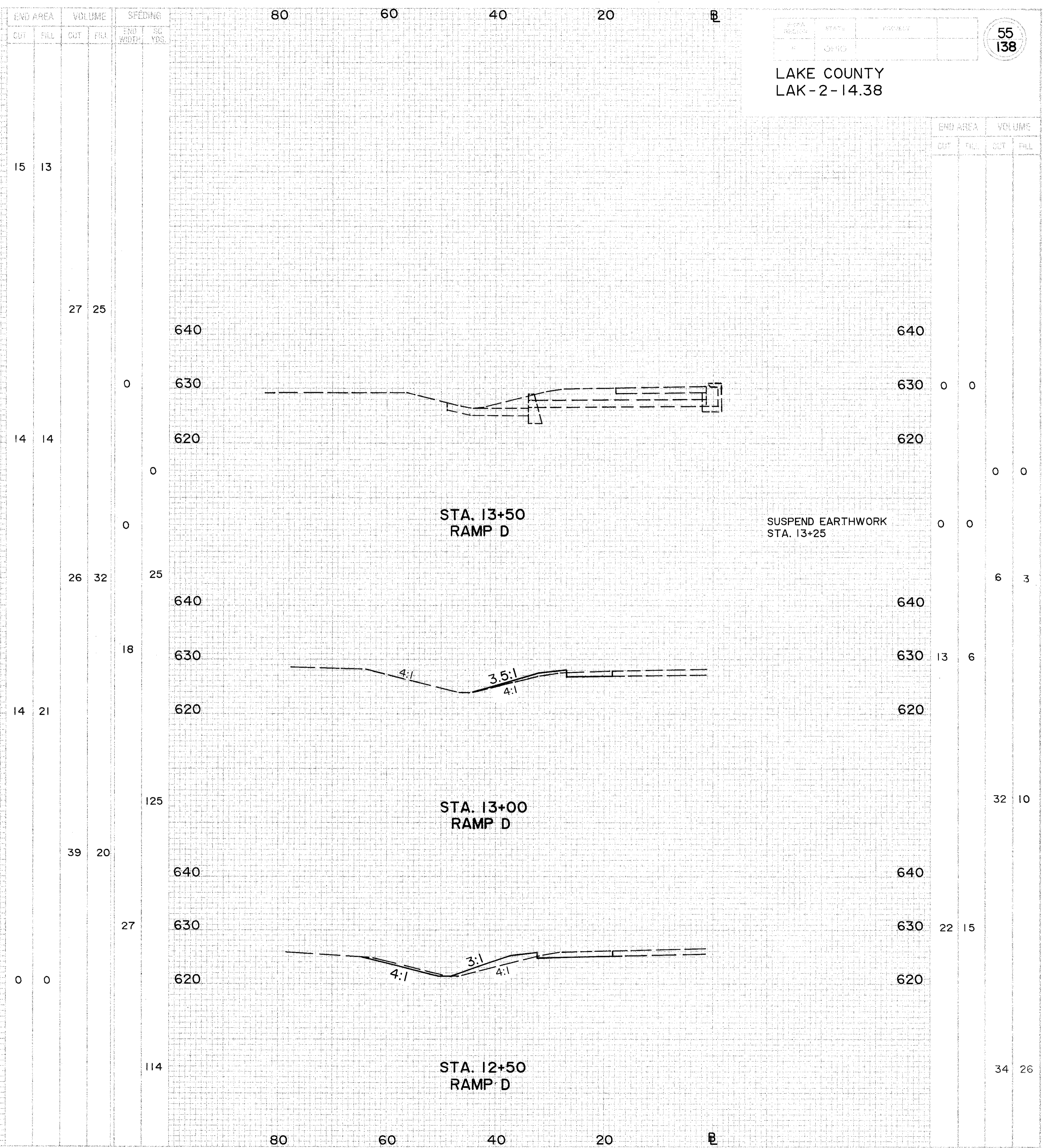
CROSS SECTIONS (RAMP D) STA. 10+50 TO STA. 13+50
