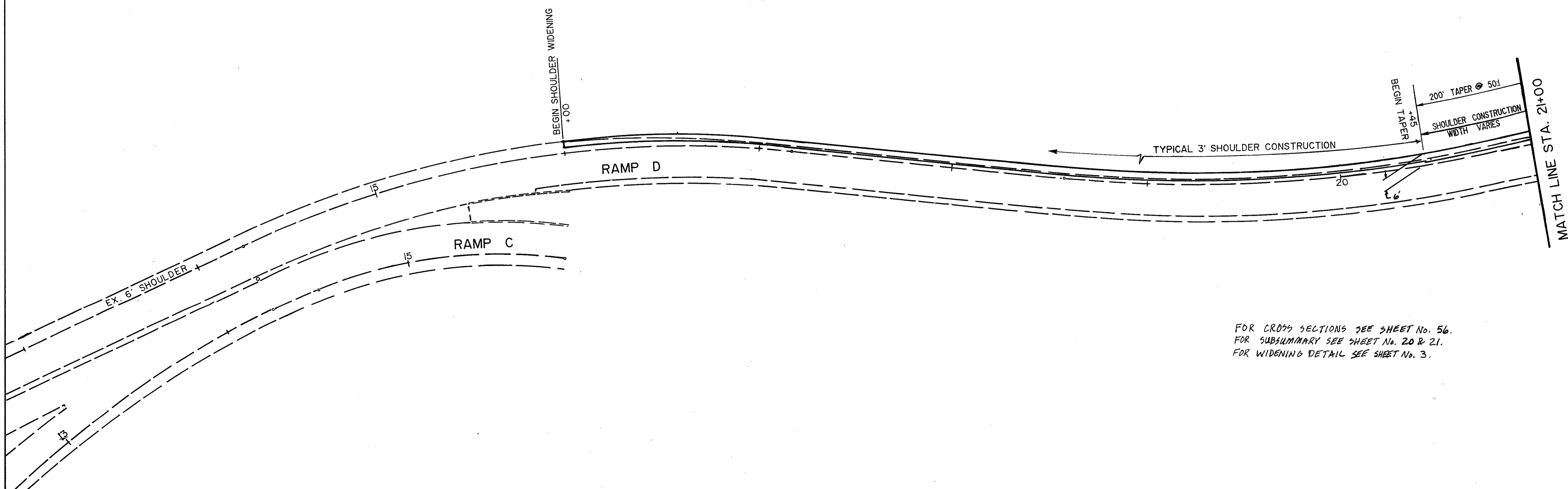
SHOULDER WIDENING TRANSITION - RAMP D
