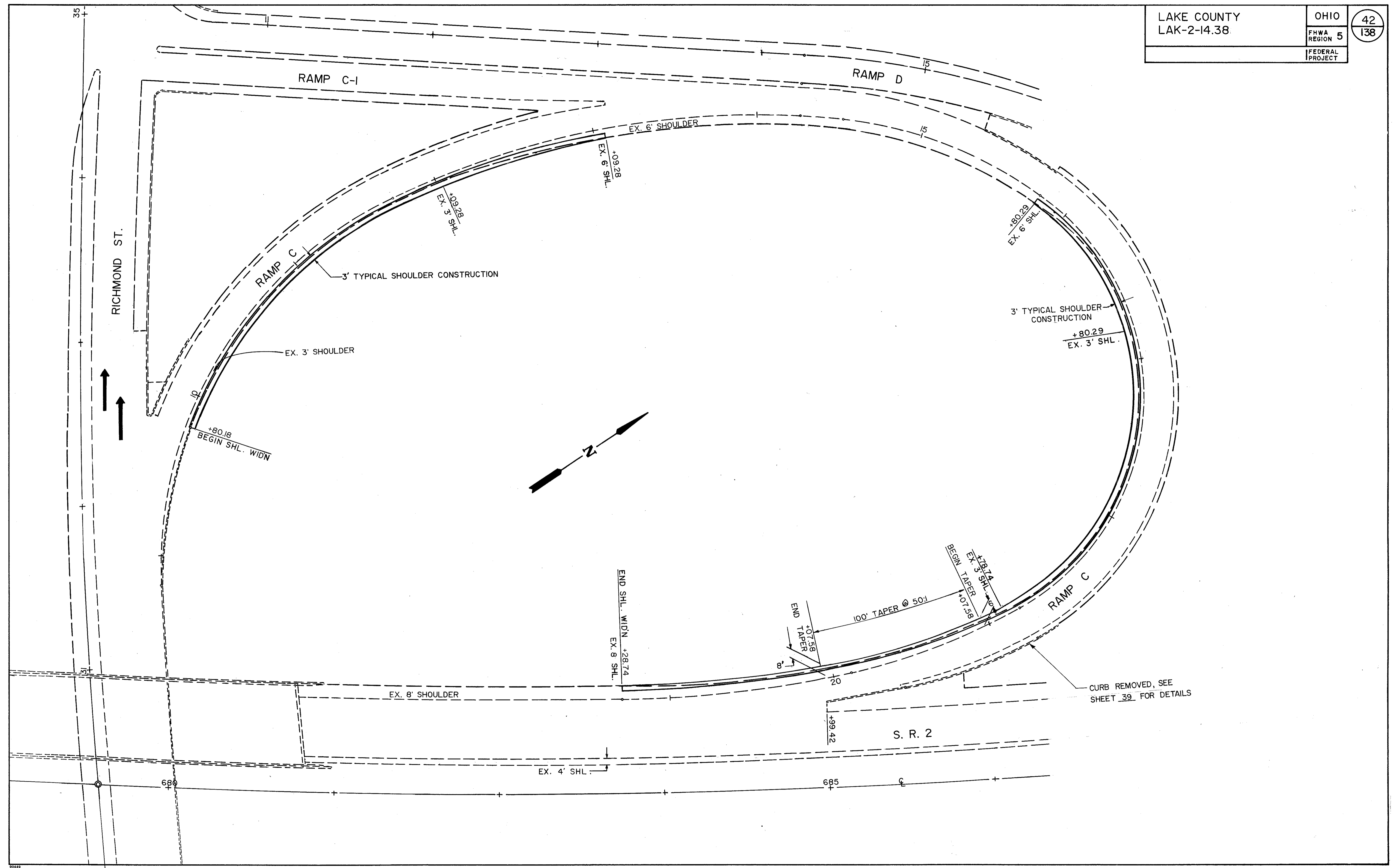
SHOULDER WIDENING TRANSITION - RAMP C
