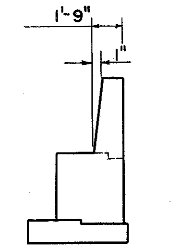
BACK WALL SLOPE Abutment-2 only
