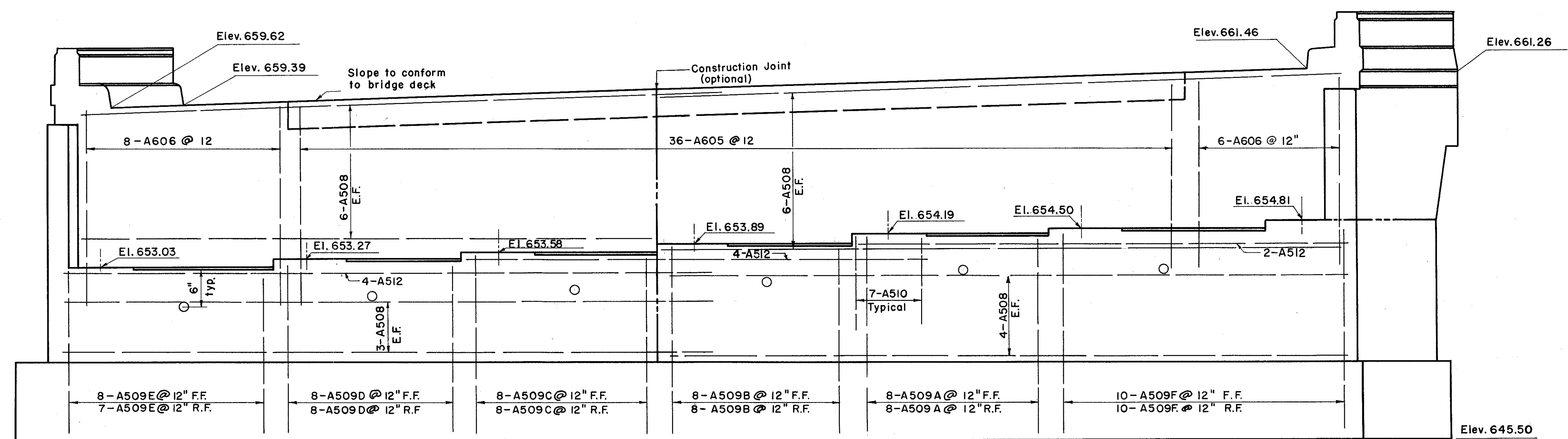
ELEVATION (Piles not shown see abut. details)
