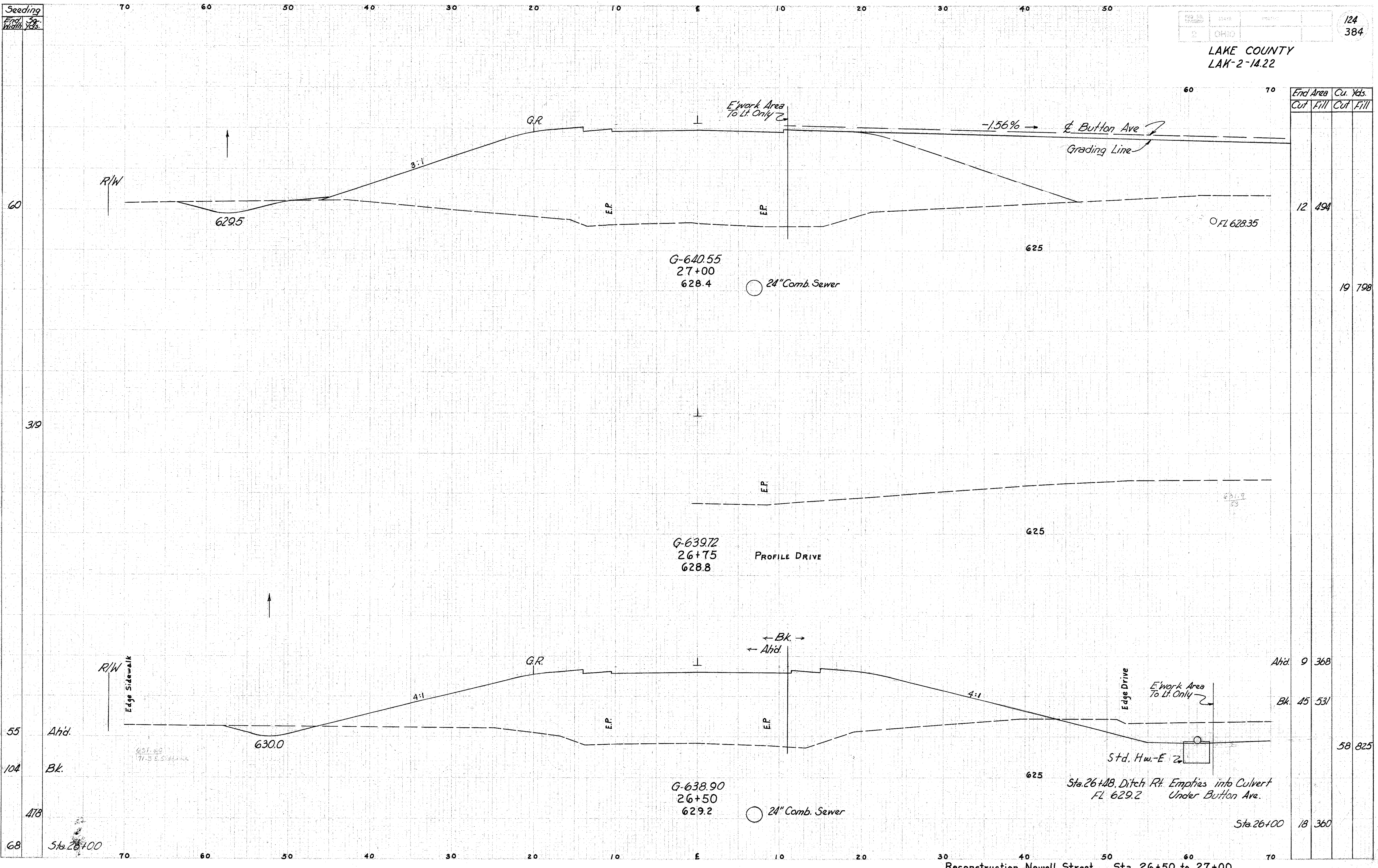
Reconstruction Newell Street Sta. 26+50 to 27+00
