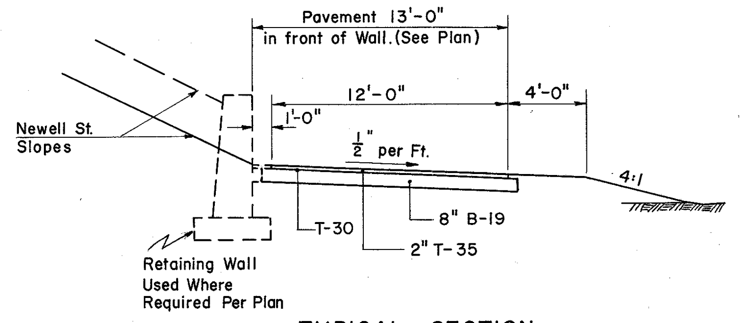
TYPICAL SECTION FRONTAGE ROAD WEST & EAST
