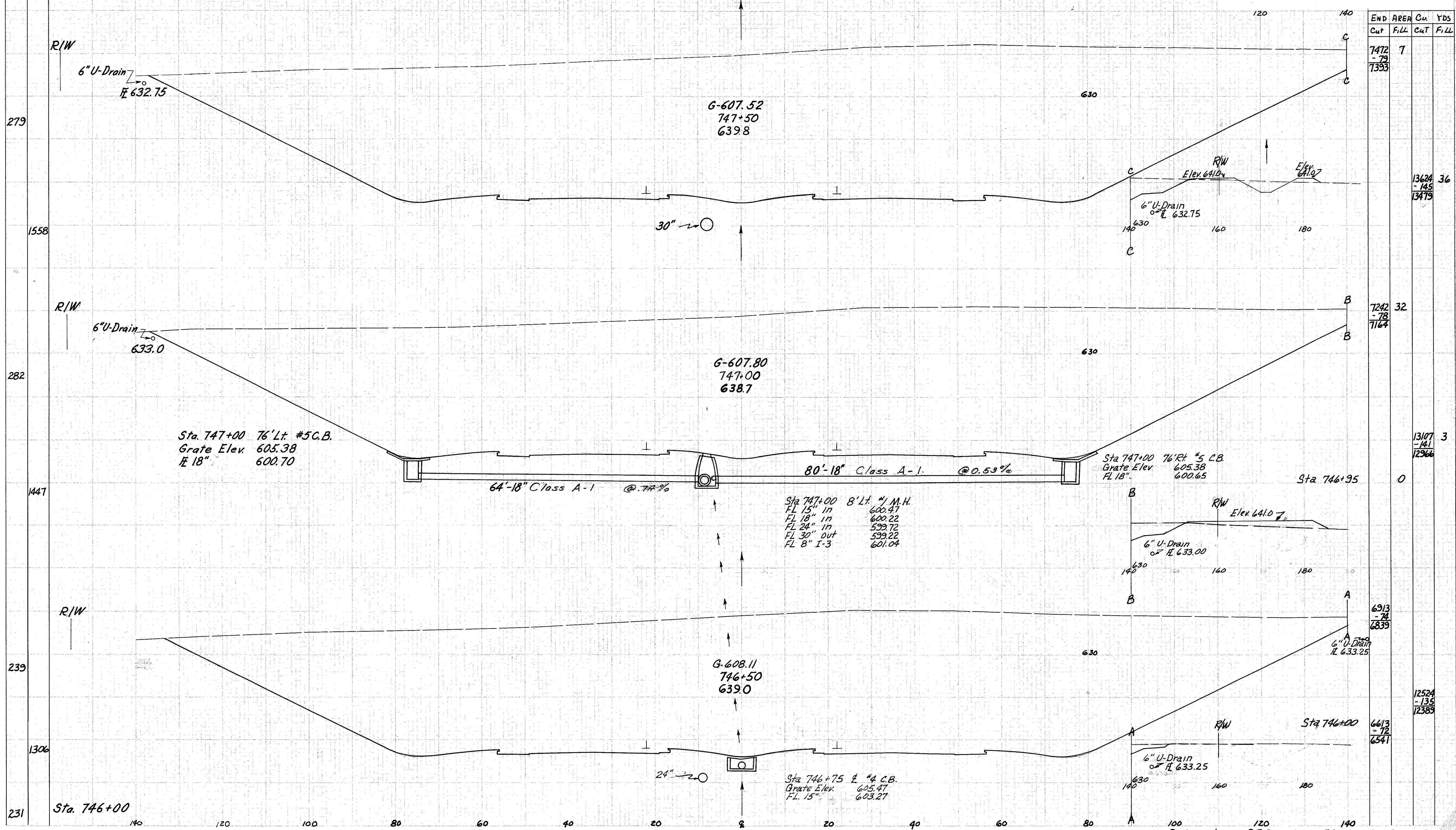
Relocation SR2 Sta. 746+50 to 747+50
