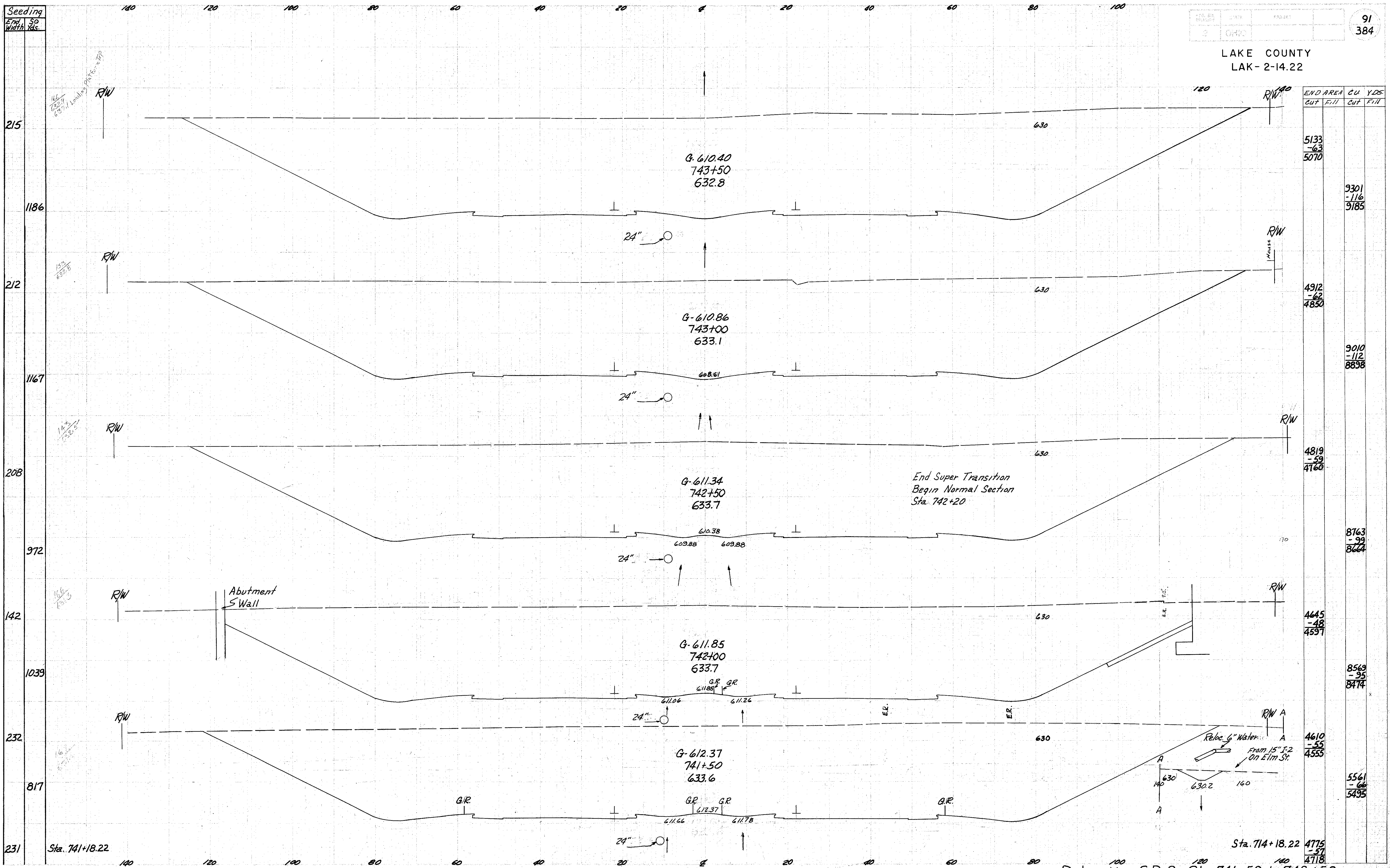
Relocation S.R.2 Sta. 741+50 to 743+50
