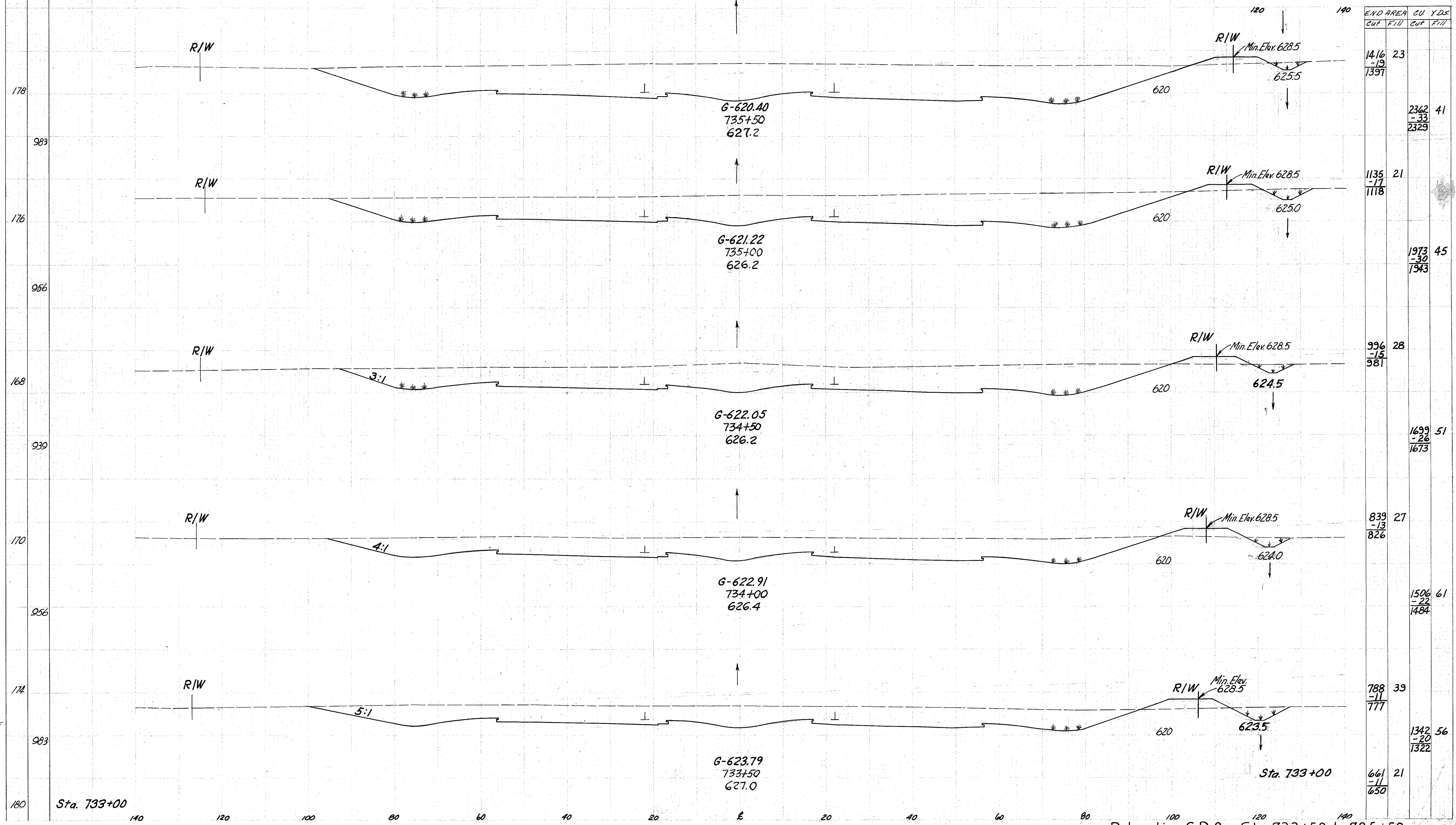
Relocation S.R.2 Sta. 733+50 to 735+50
