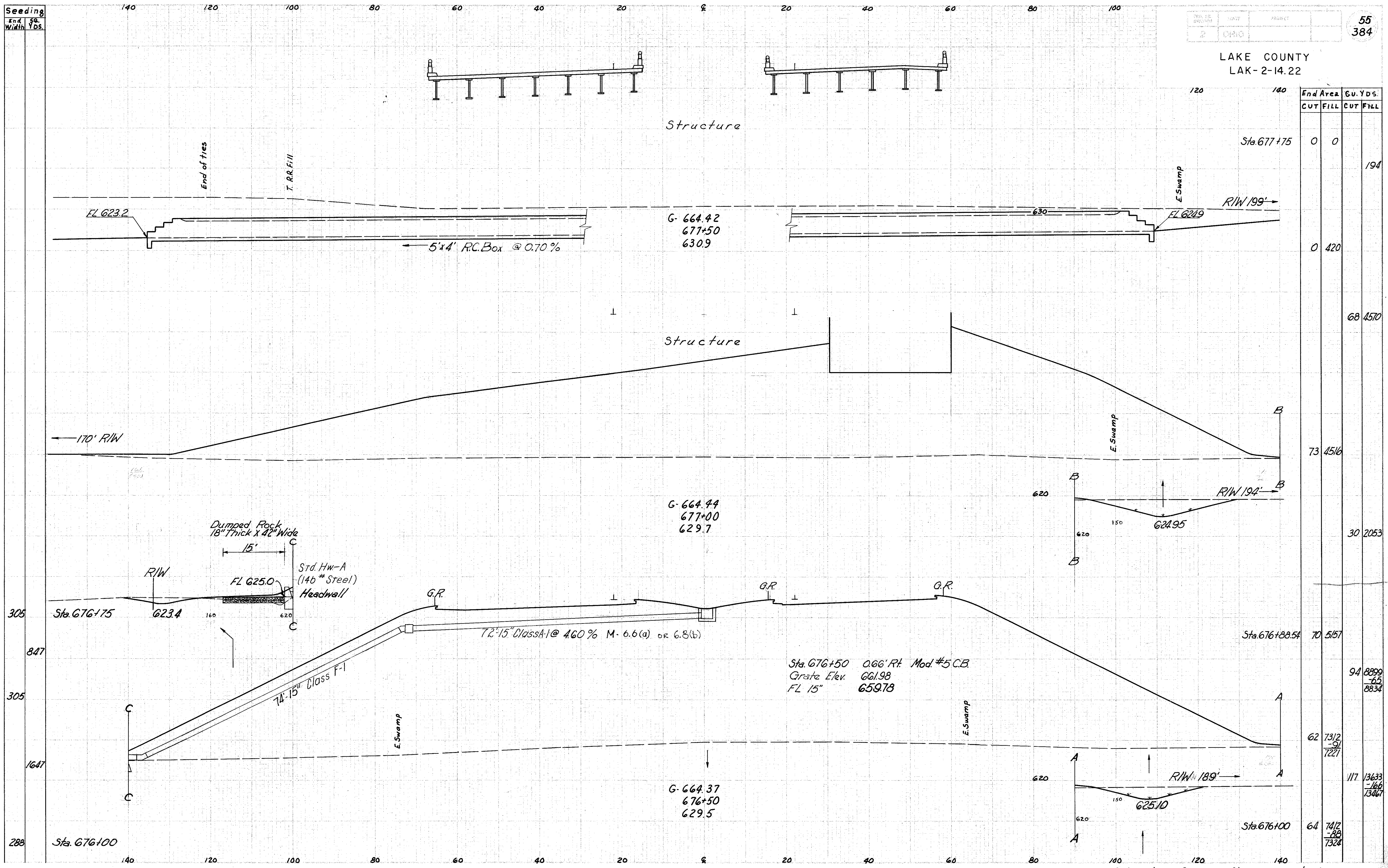
Relocation SR.2 Sta. 676+50 to 677+50
