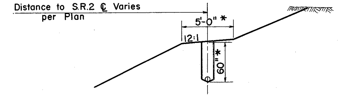
DETAIL OF CLASS I-3 PIPE ON CUT SLOPE WHERE SHOWN ON PLAN
