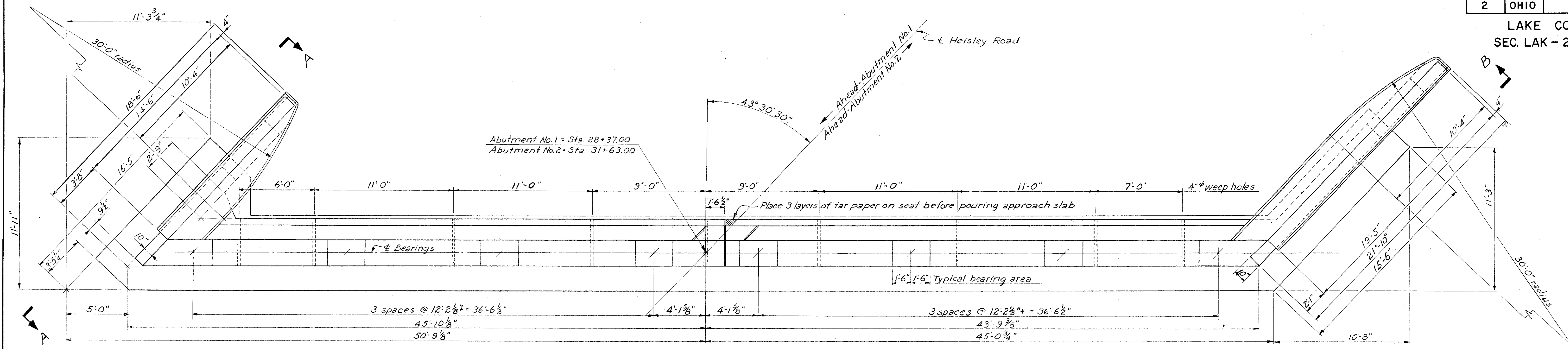
ABUTMENT PLAN
