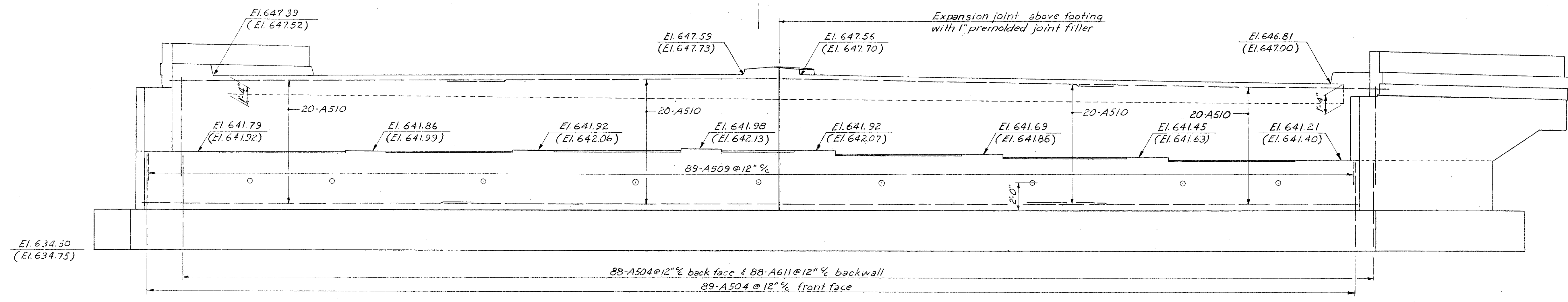
ABUTMENT ELEVATION
