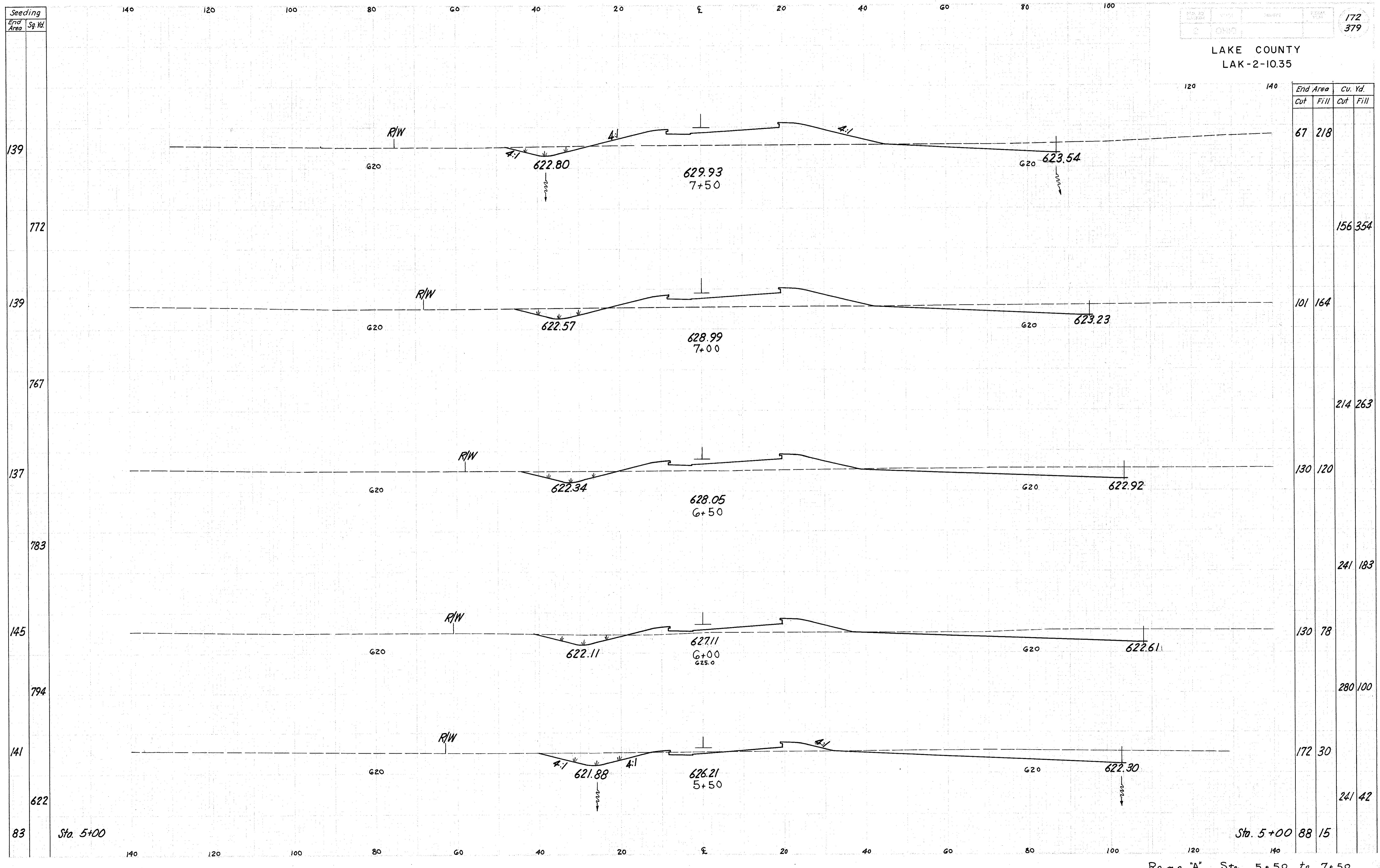
Ramp "A" Sta. 5+50 to 7+50
