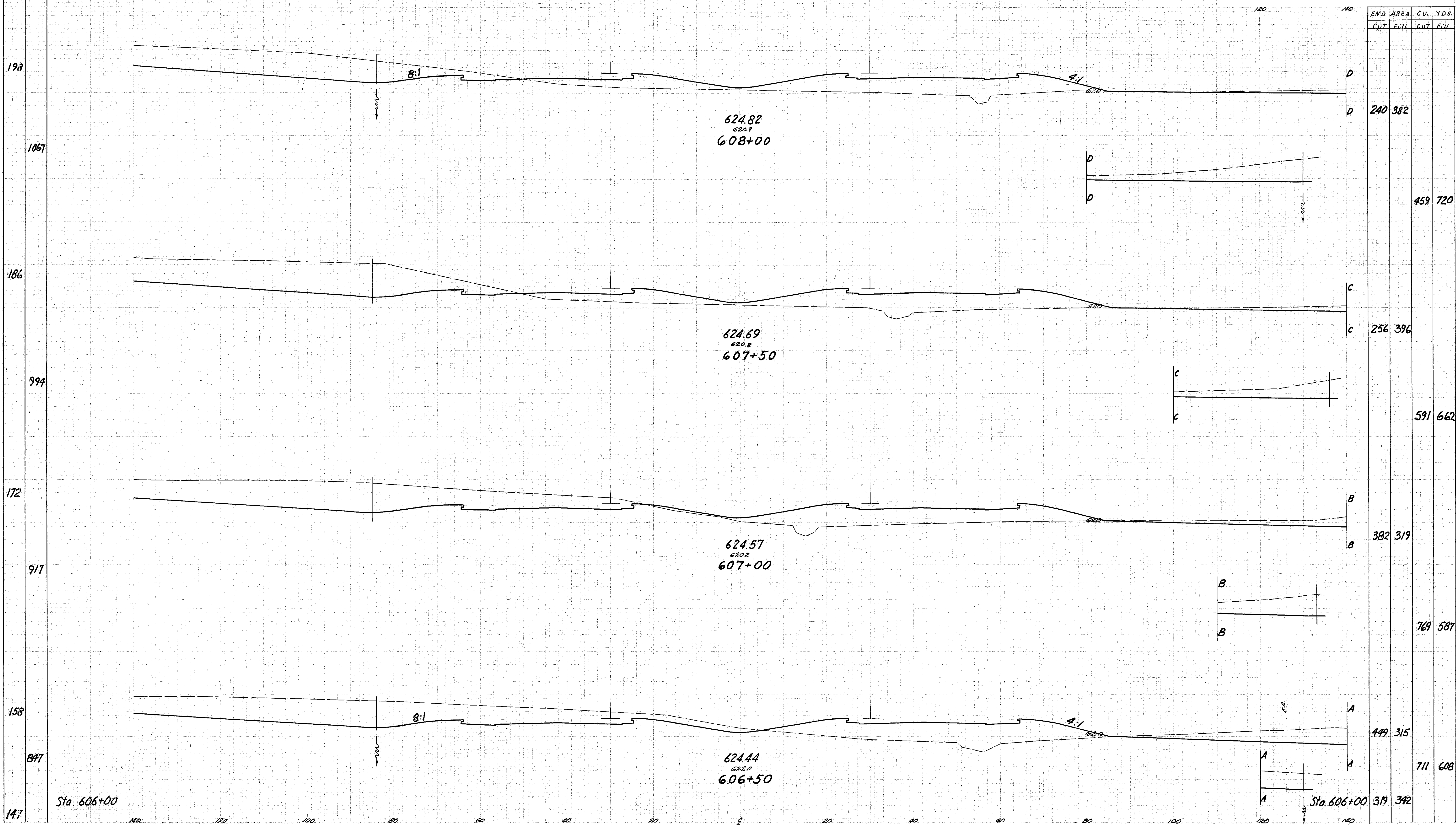
Relocation SR 2 Sta. 606+50 to 608+00
