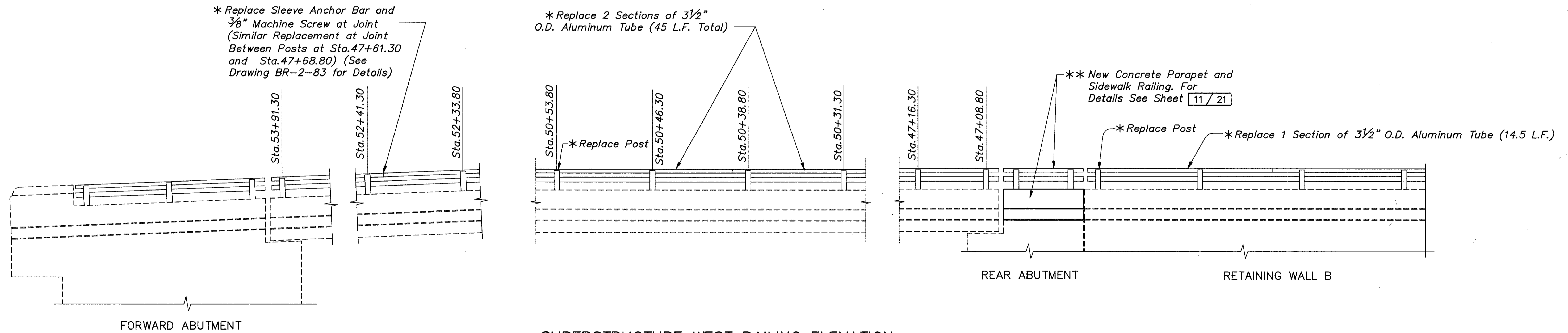
SUPERSTRUCTURE WEST RAILING ELEVATION
