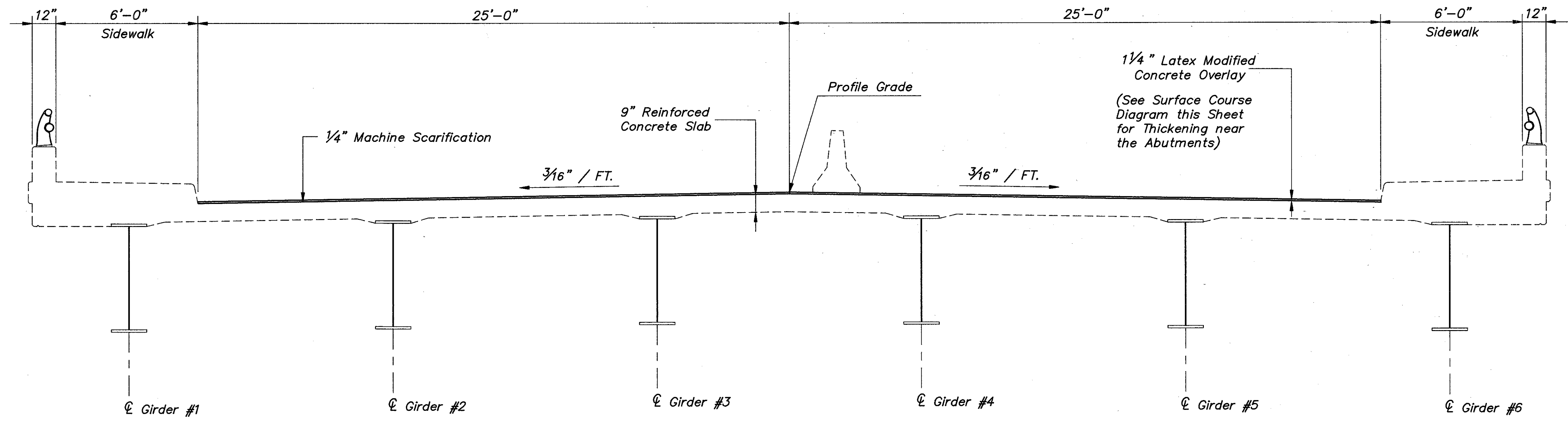
TYPICAL SECTION (LOOKING NORTH)
