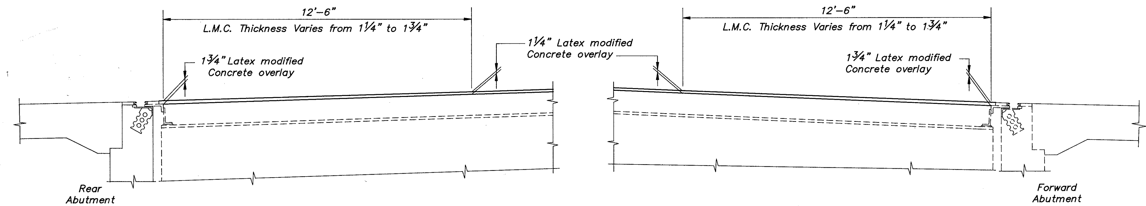
SURFACE COURSE DIAGRAM
