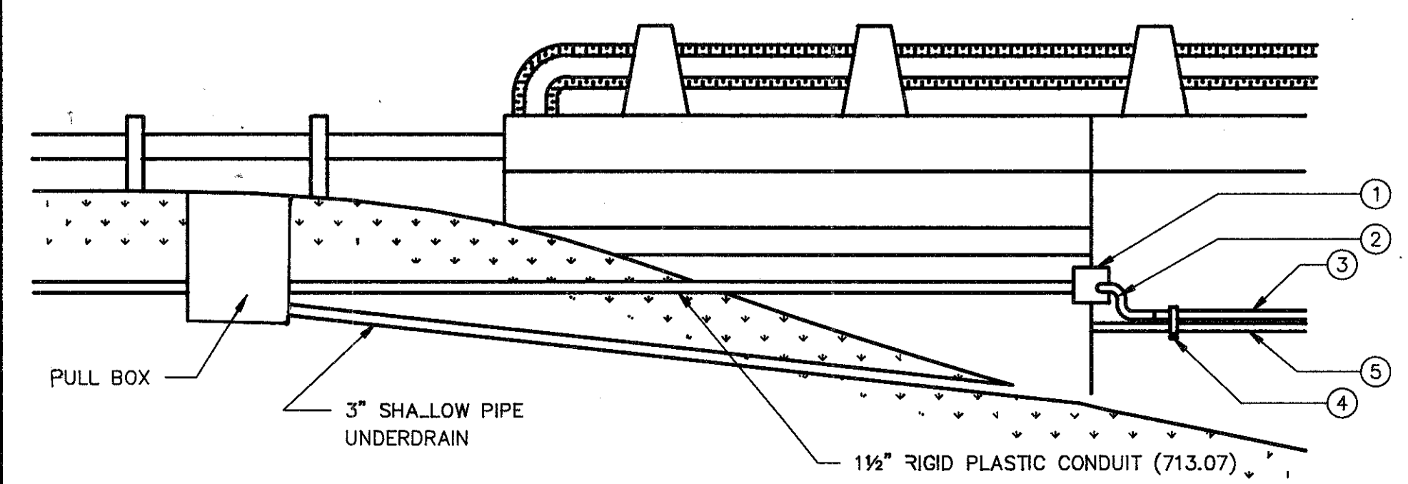
SCHEMATIC FOR INTERCONNECT BRIDGE CONNECTION SKETCH NOT TO SCALE
