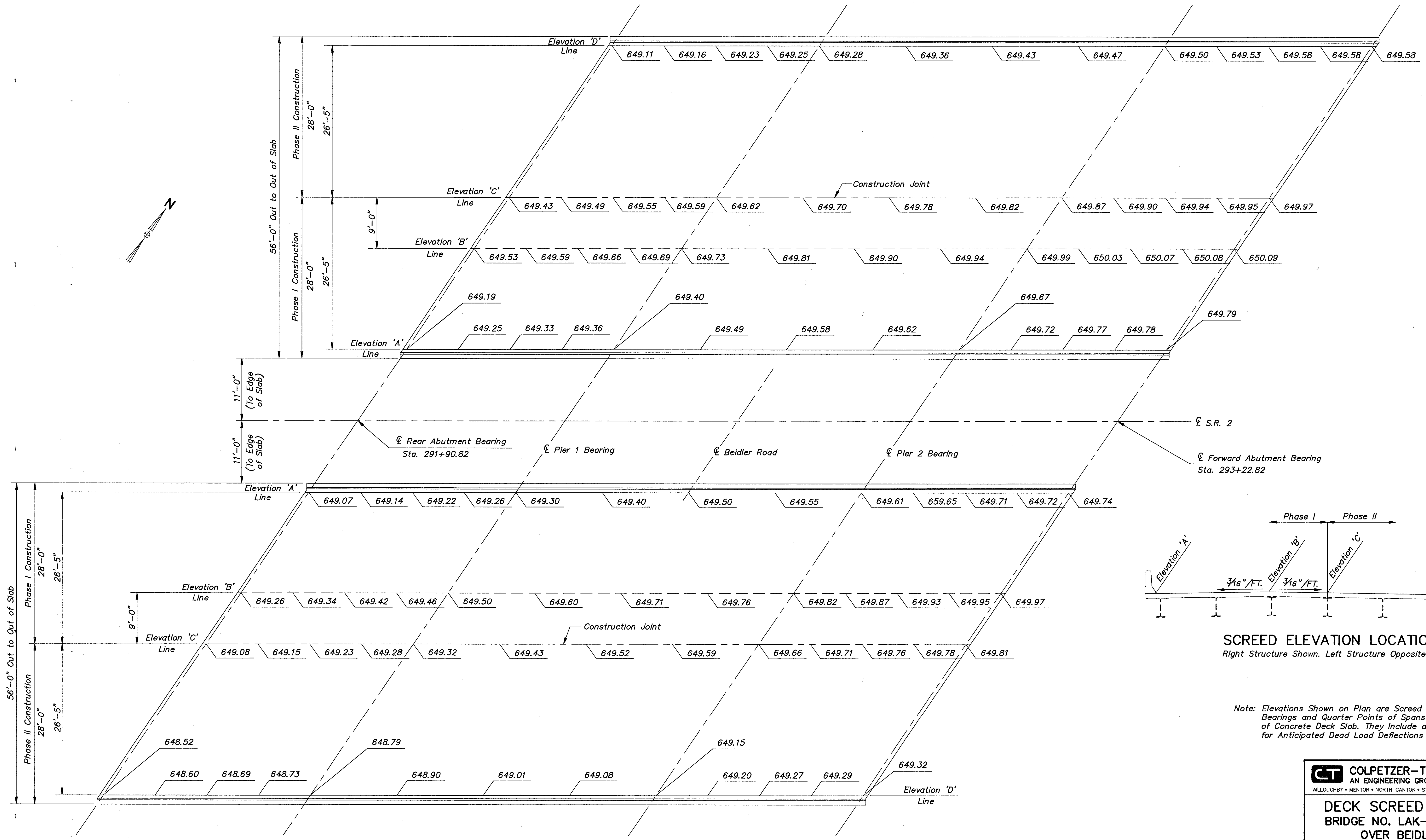
PLAN-DECK SCREED ELEVATIONS
