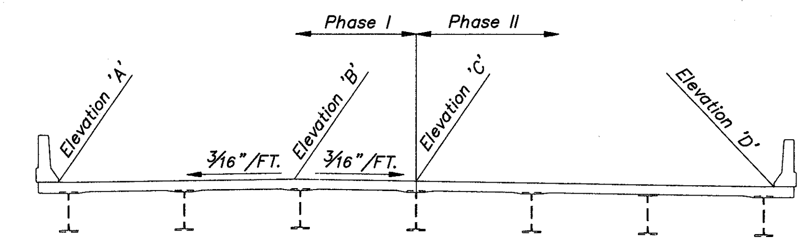
SCREED ELEVATION LOCATIONS Right Structure Shown. Left Structure Opposite Hand.
