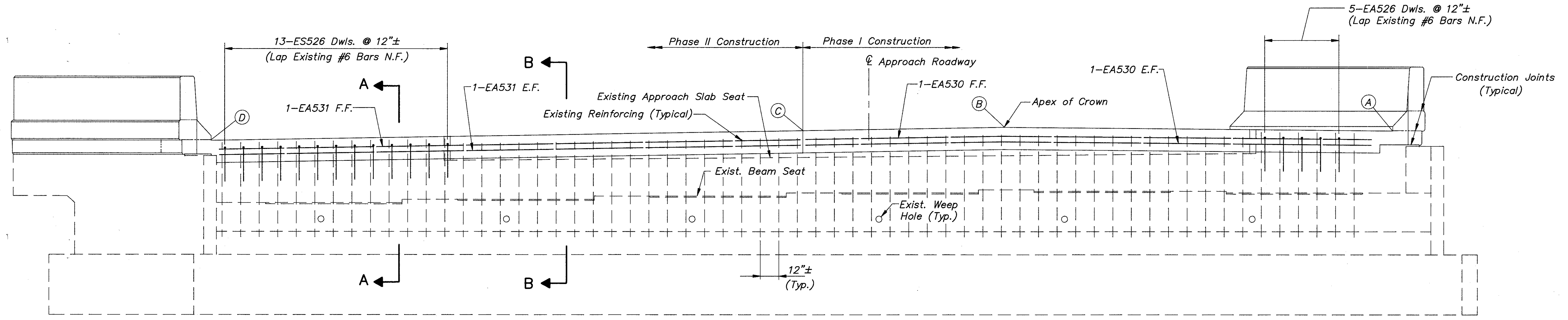
PLAN ABUTMENT BACKWALL CAPPING (TYPICAL FOR ABUTMENTS RR AND LF)
