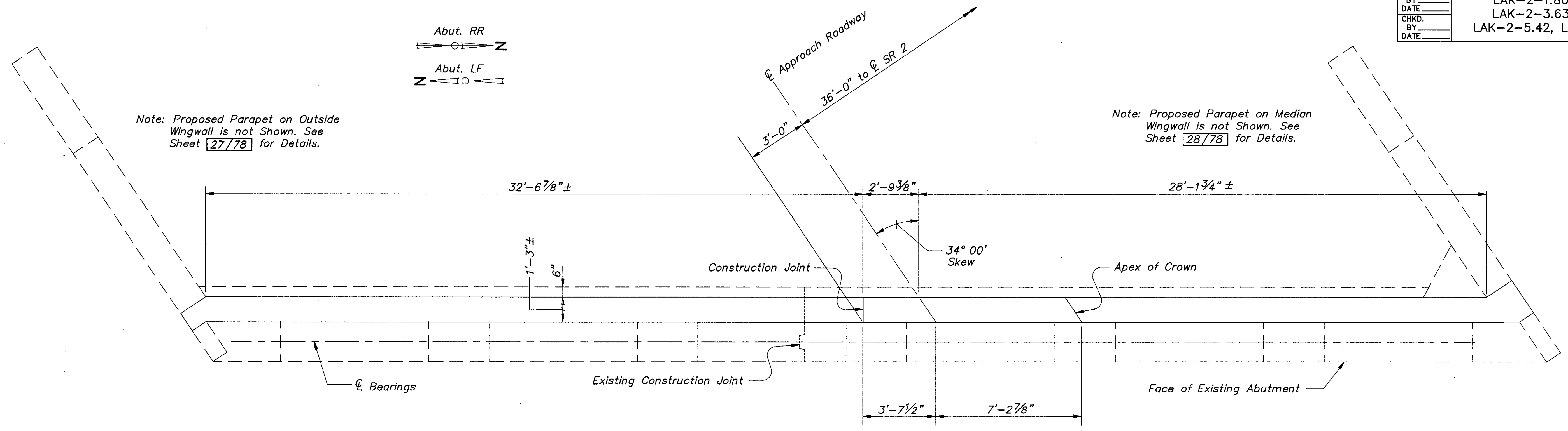
PLAN ABUTMENT BACKWALL CAPPING (TYPICAL FOR ABUTMENTS RR AND LF)
