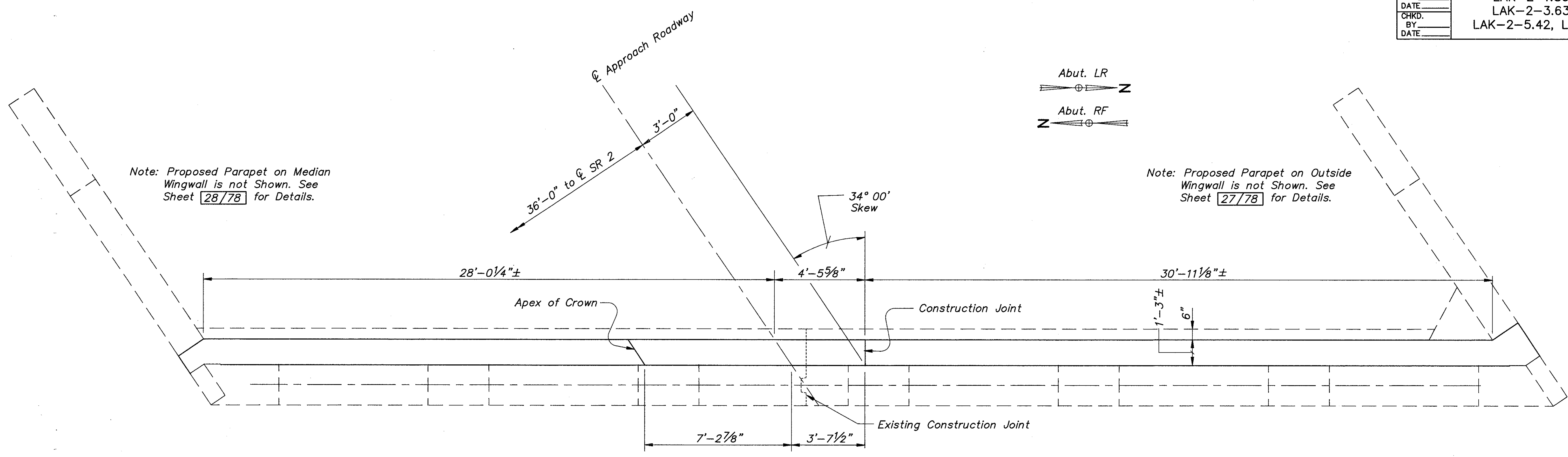
PLAN ABUTMENT BACKWALL CAPPING (TYPICAL FOR ABUTMENTS LR AND RF)
