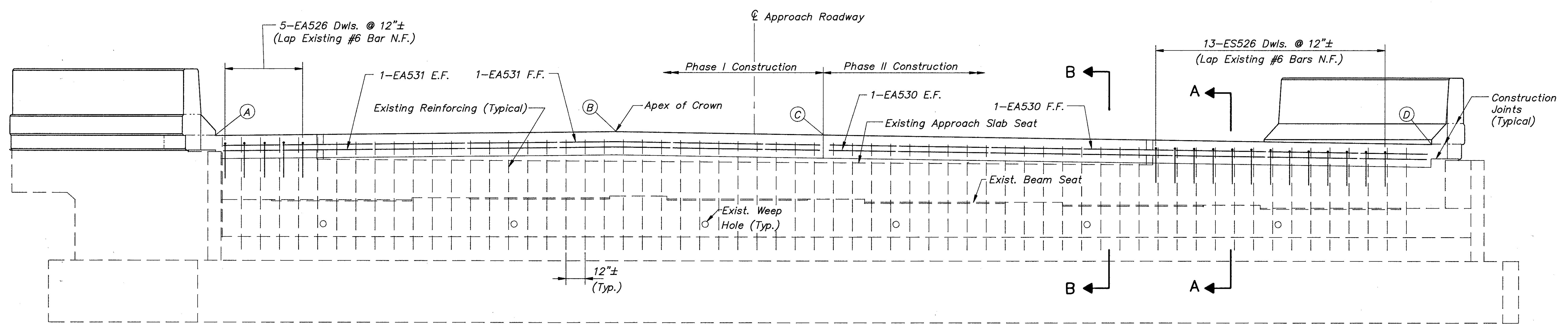
ELEVATION ABUTMENT BACKWALL CAPPING (TYPICAL FOR ABUTMENTS LR AND RF)
