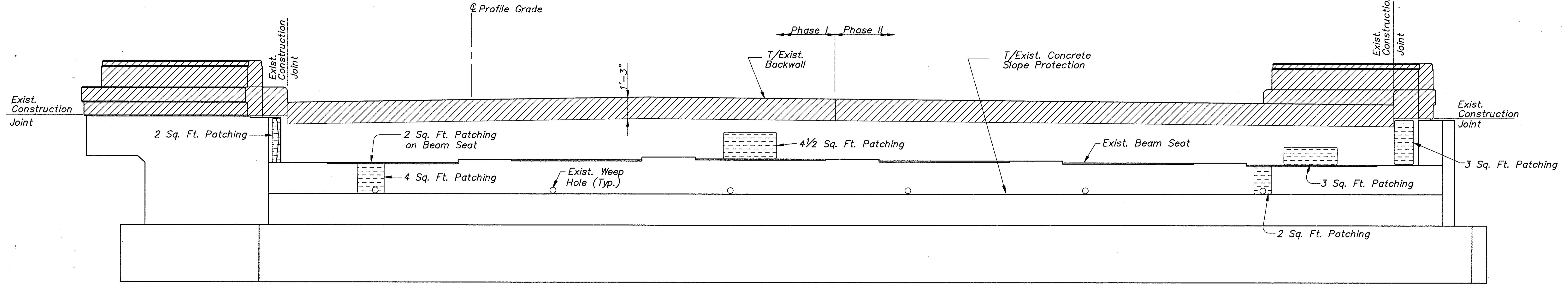
ELEVATION REAR ABUTMENT
