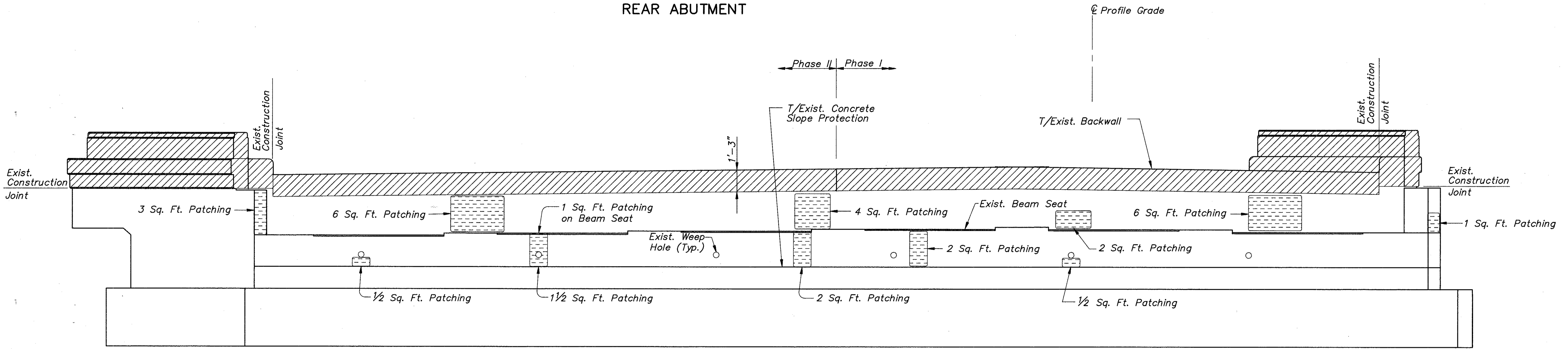
ELEVATION FORWARD ABUTMENT
