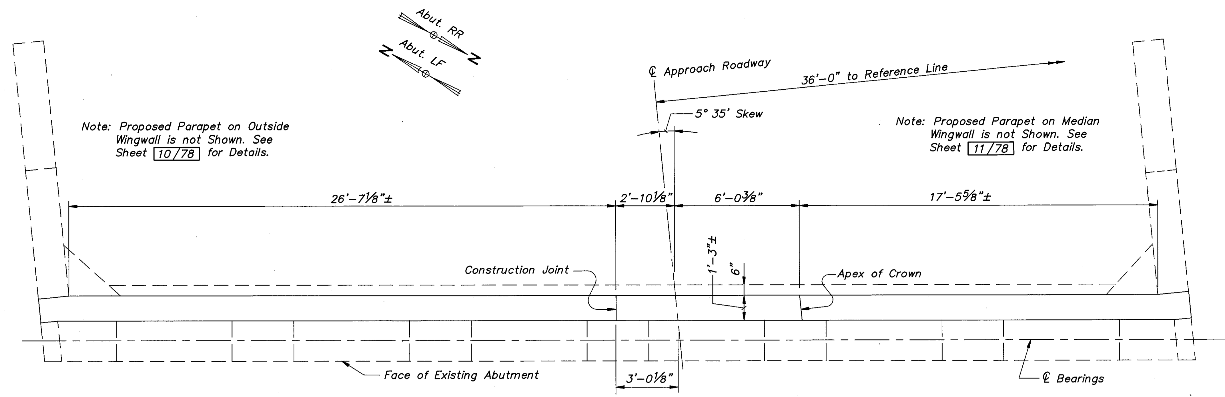
PLAN ABUTMENT BACKWALL CAPPING (TYPICAL FOR RR AND LF ABUTMENTS)
