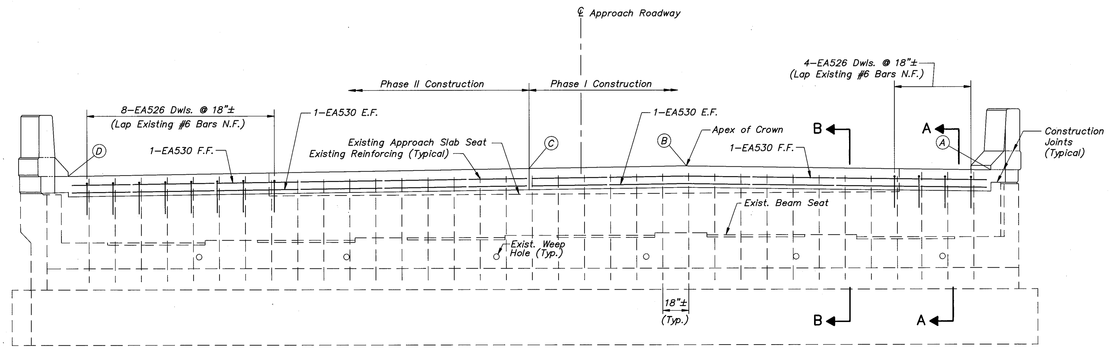
ELEVATION ABUTMENT BACKWALL CAPPING (TYPICAL FOR RR AND LF ABUTMENTS)
