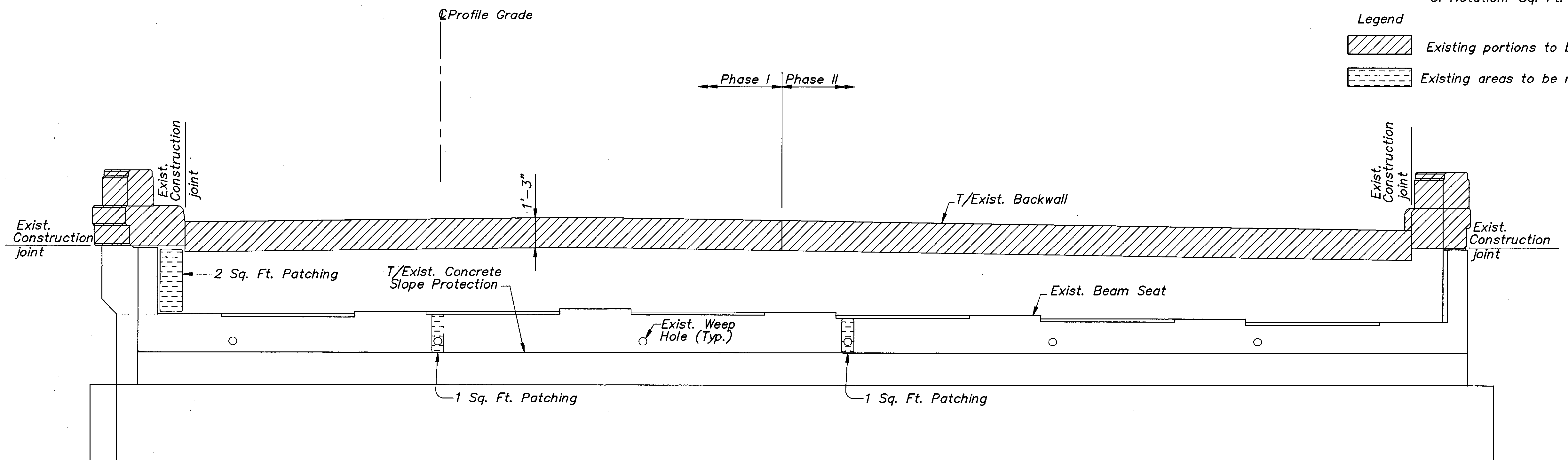
ELEVATION FORWARD ABUTMENT
