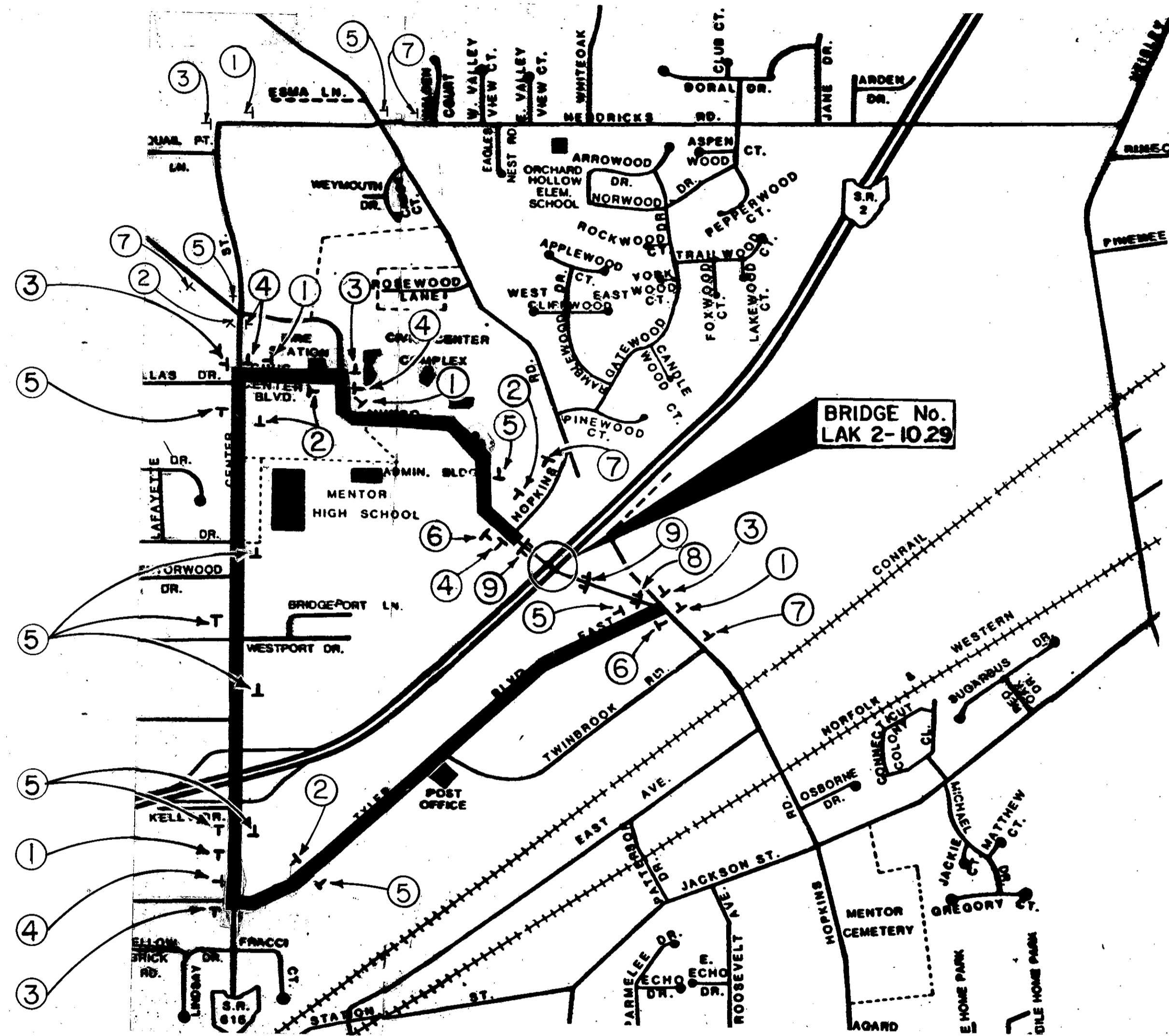
DETOUR PLAN no scale
