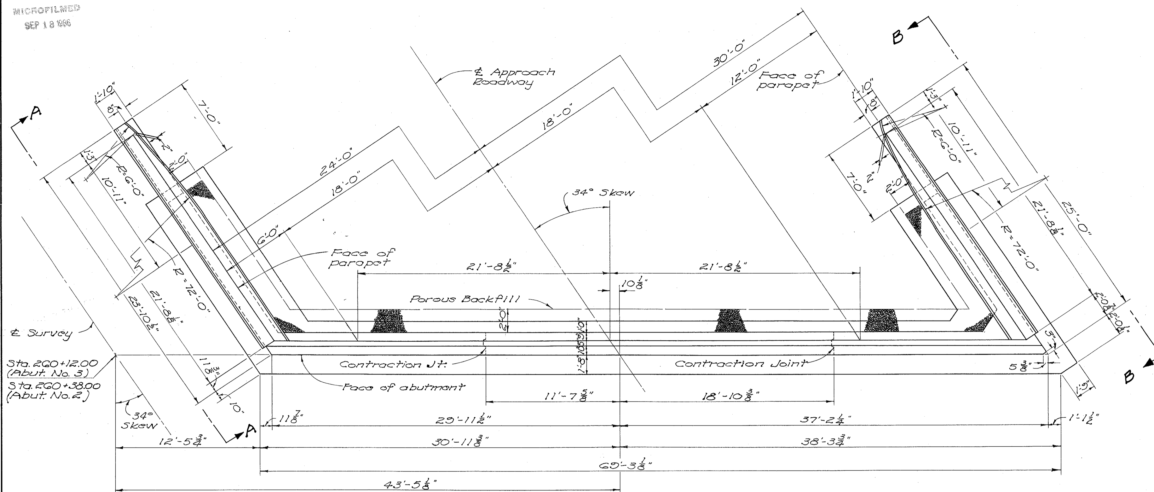
ABUTMENT PLAN (Abutments No. 2 and No. 3)
