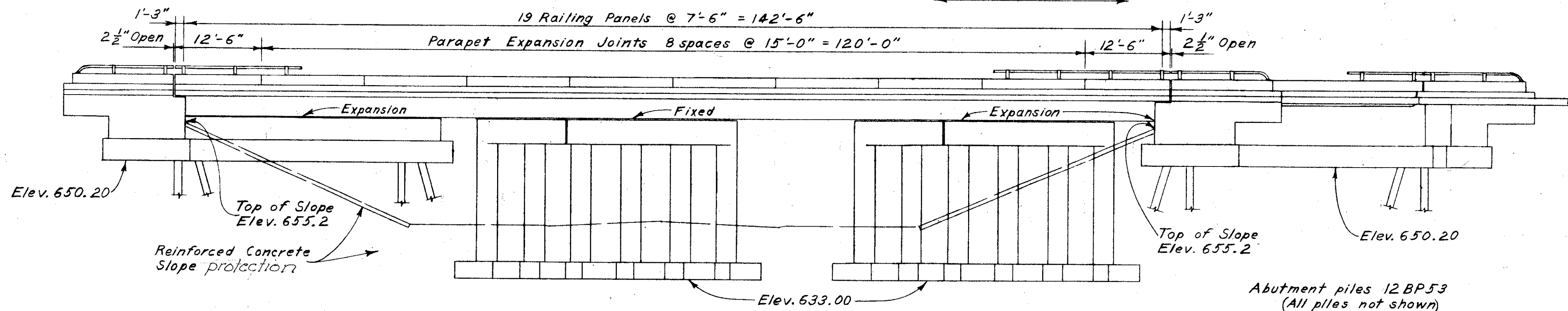
GENERAL ELEVATION
