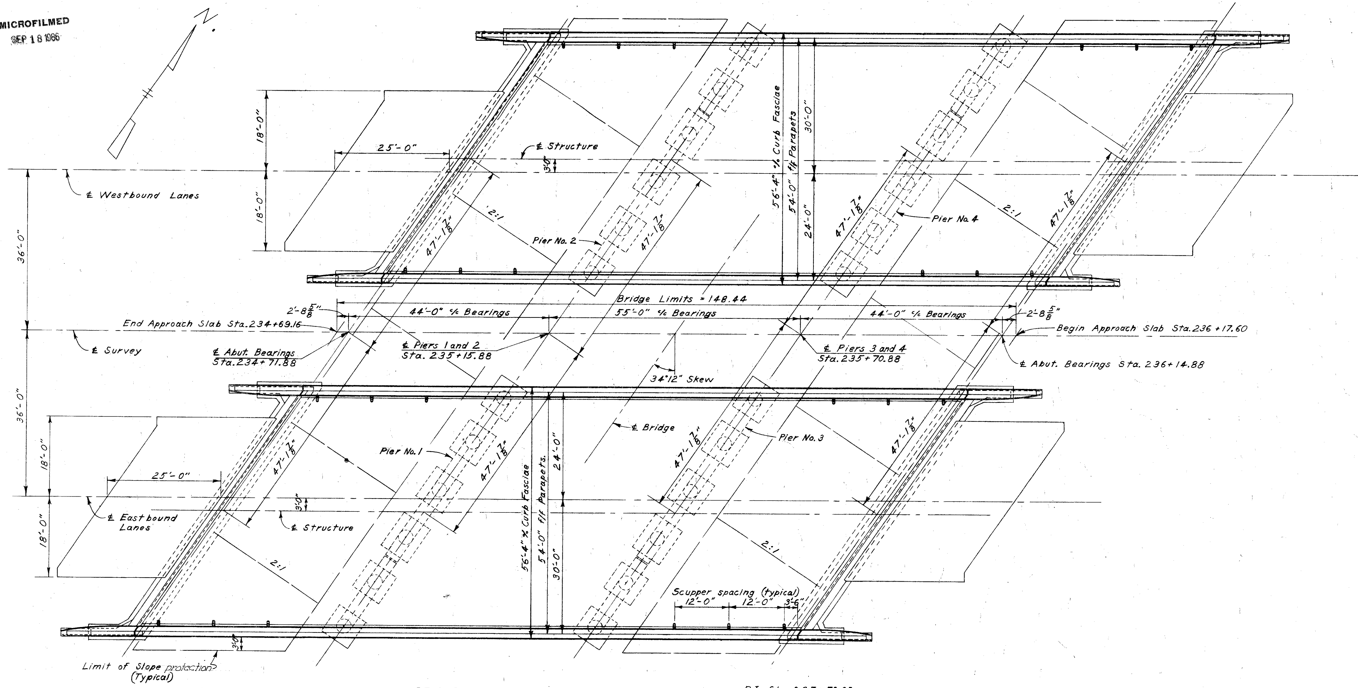
GENERAL PLAN
