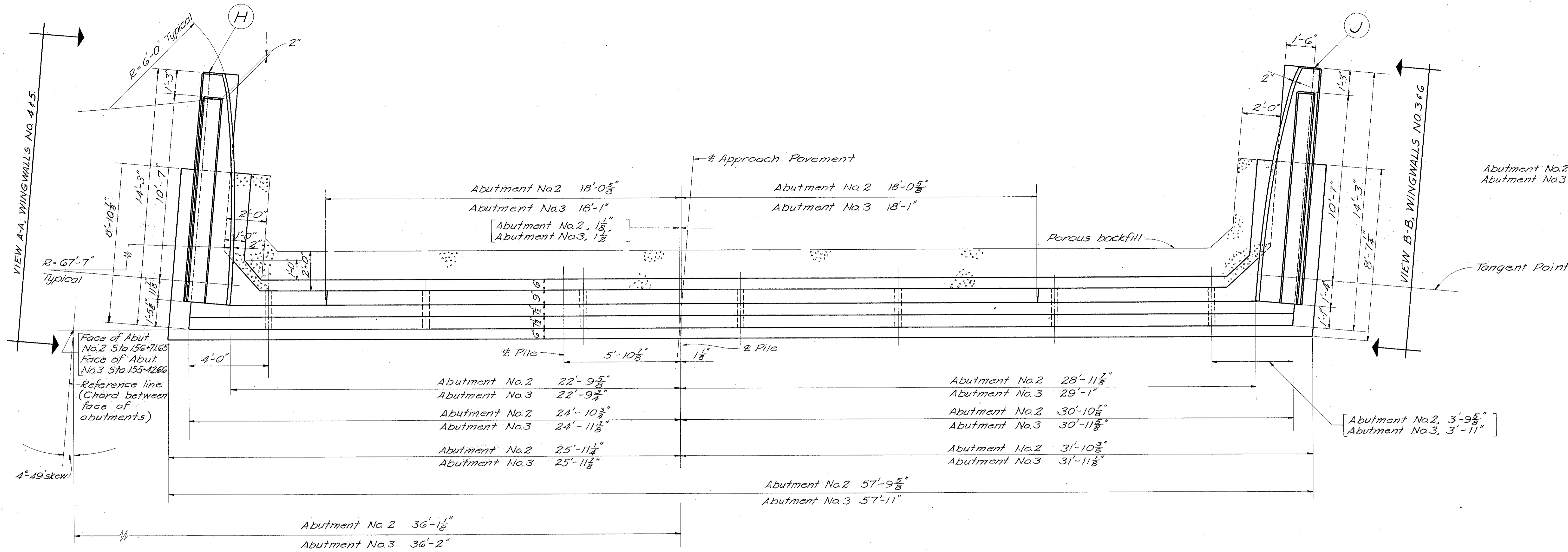
PLAN (Wing Walls to be parallel to Reference line)
