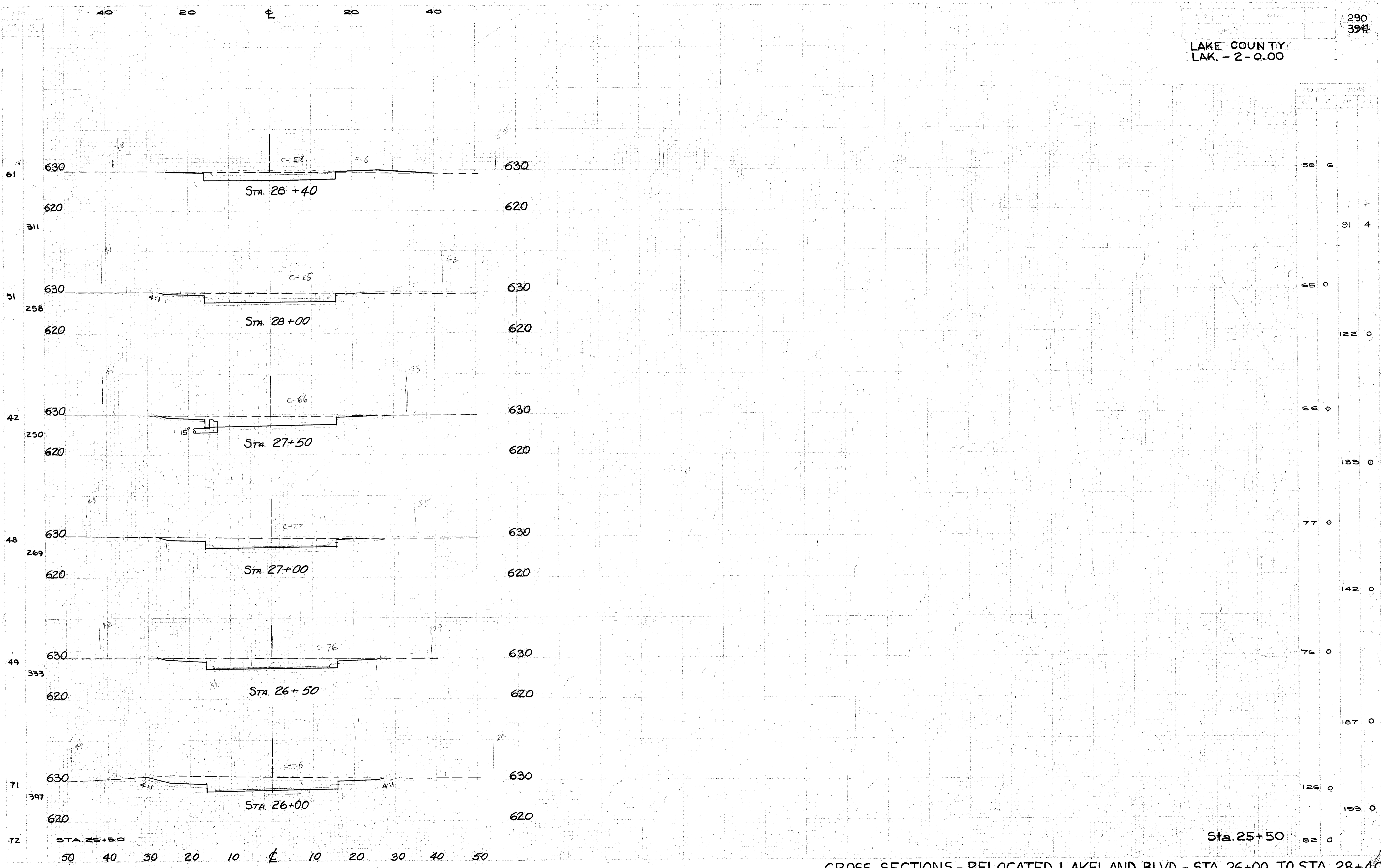
CROSS SECTIONS - RELOCATED LAKELAND BLVD. - STA. 26+00 TO STA. 28+40
