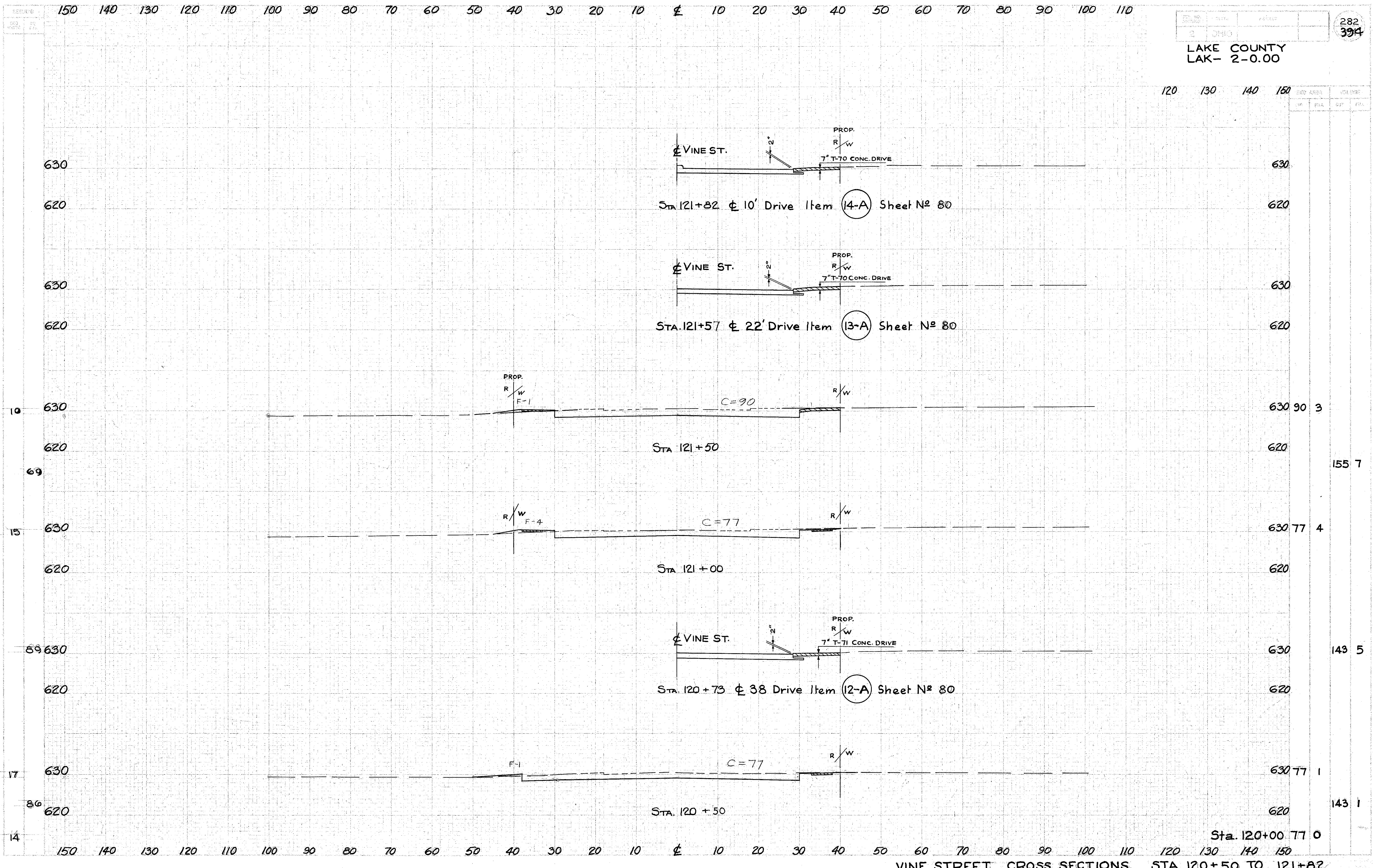
VINE STREET CROSS SECTIONS STA 120+50 TO 121+82
