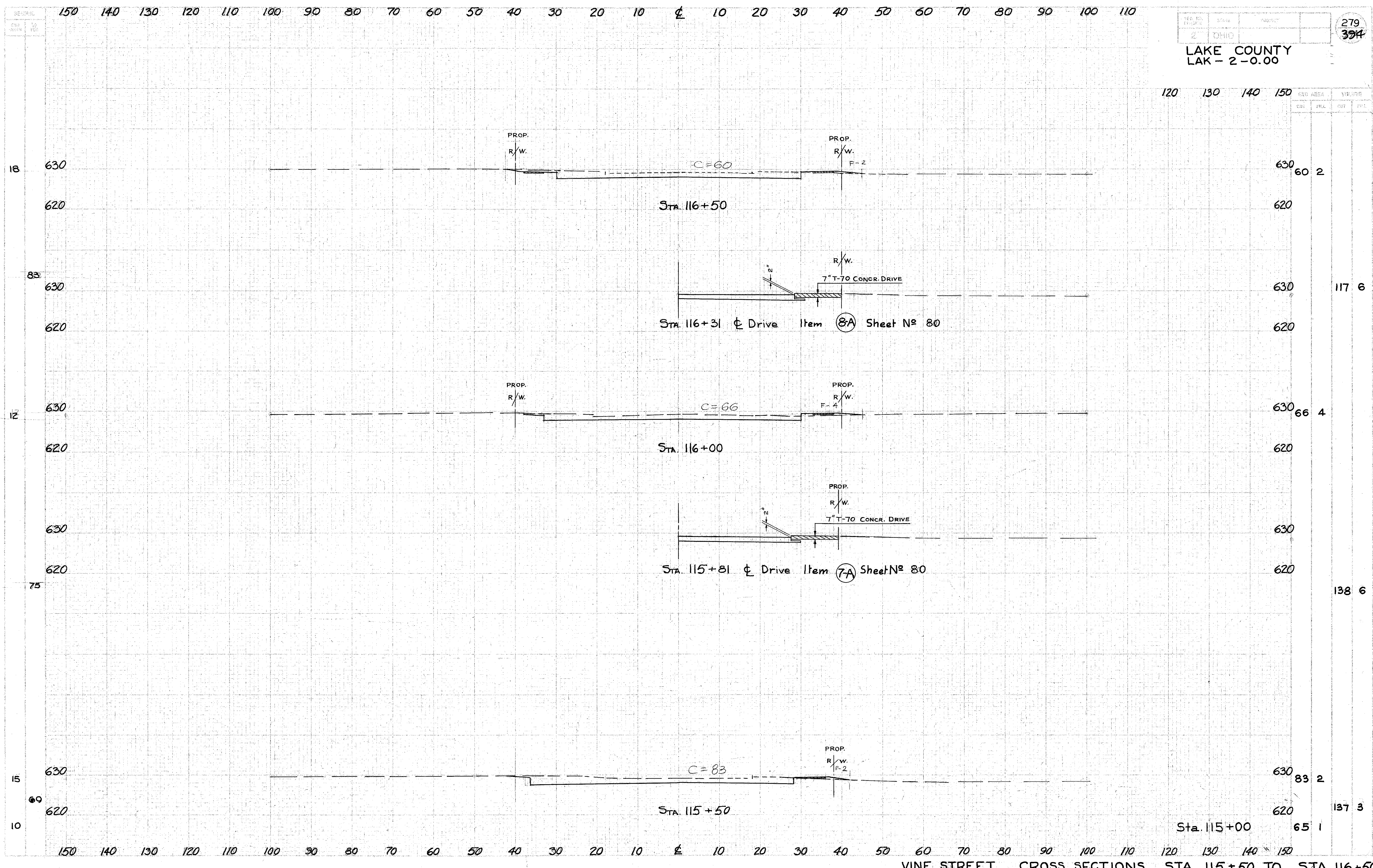
VINE STREET CROSS SECTIONS STA. 115+50 TO STA. 116+50
