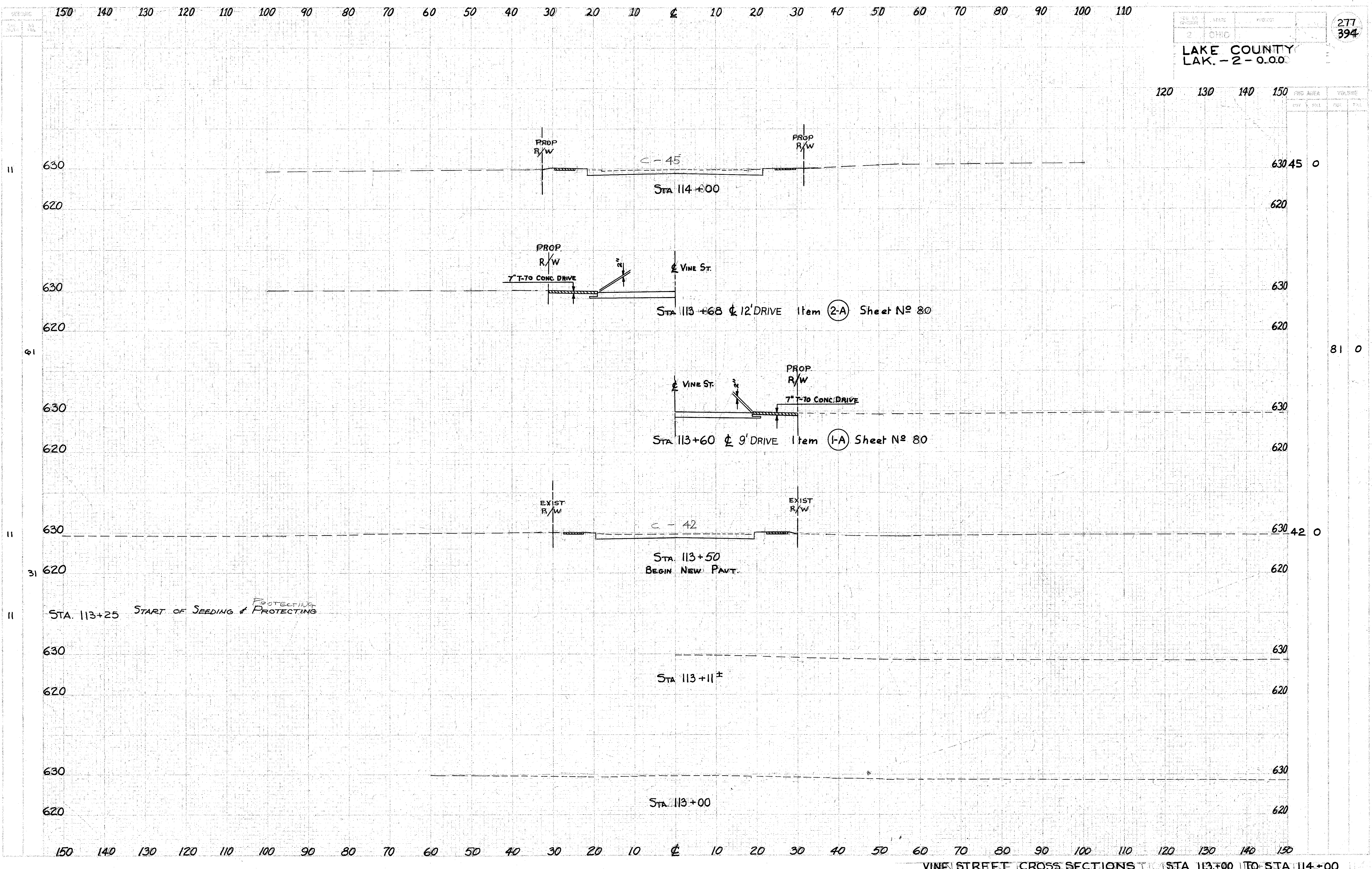
VINE STREET CROSS SECTIONS TO STA. 113+00 TO STA. 114+00
