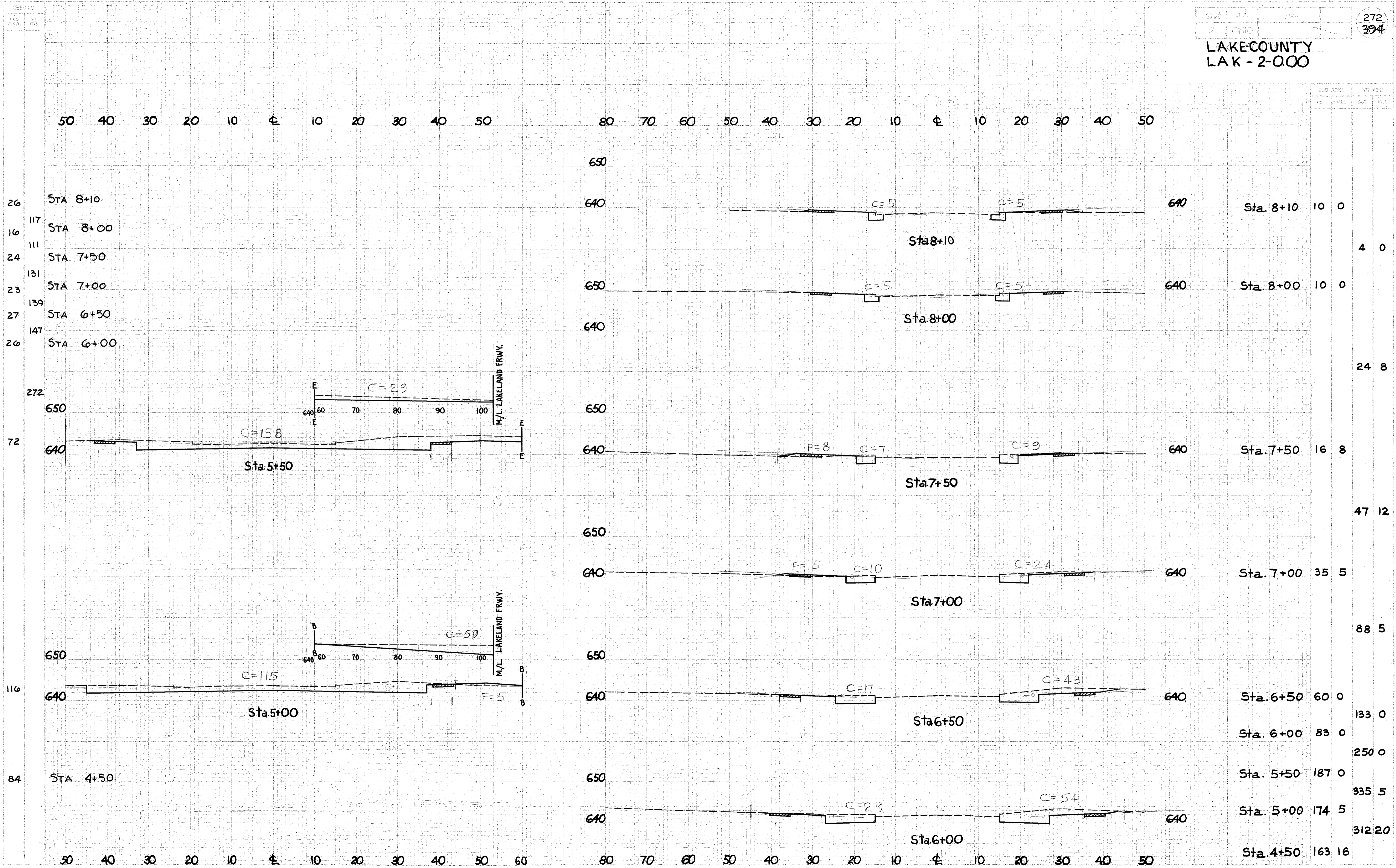
RUSH ROAD CROSS SECTIONS STA. 5+00 TO STA. 8+10
