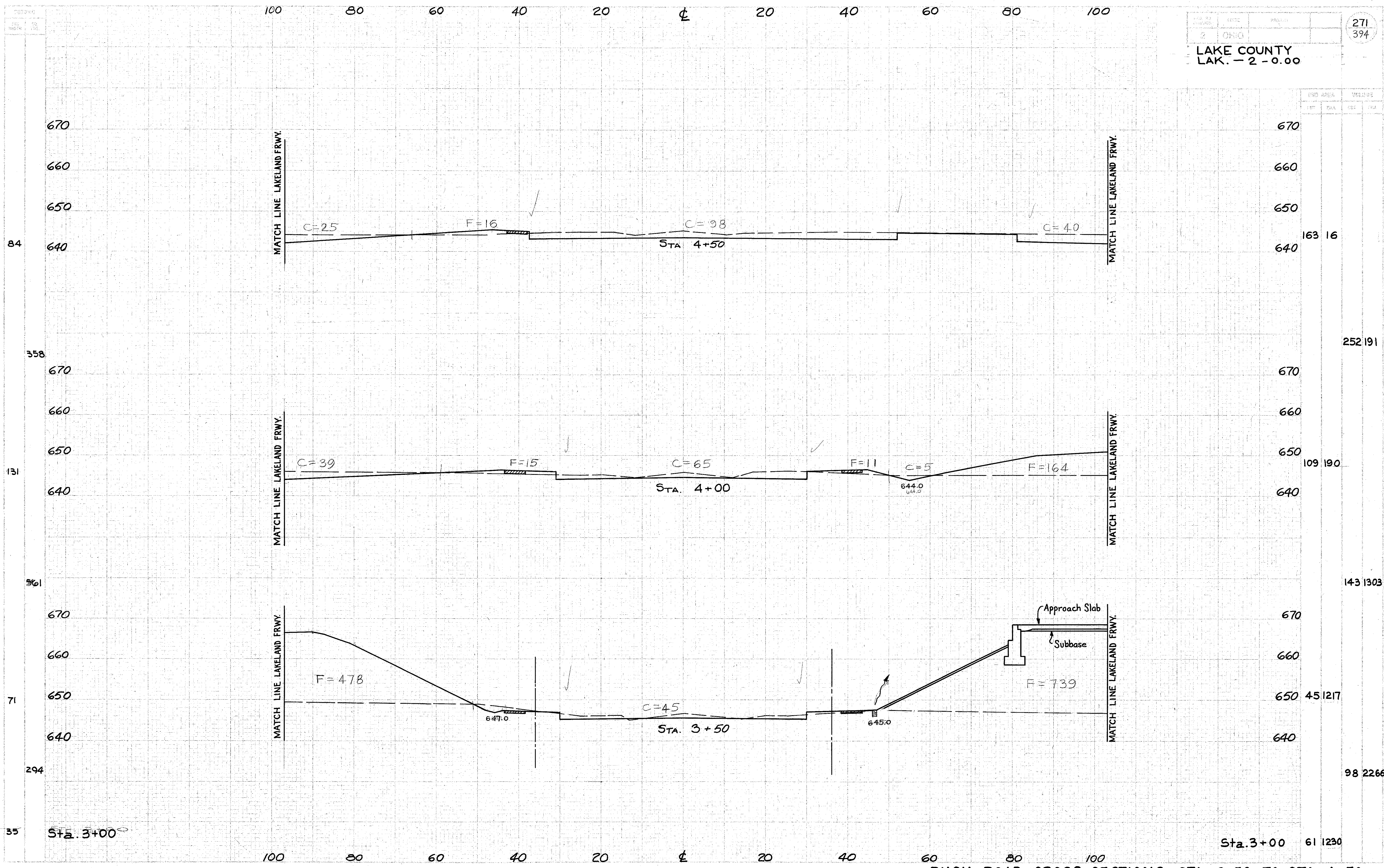
RUSH ROAD CROSS SECTIONS STA. 3+50 TO STA. 4+50
