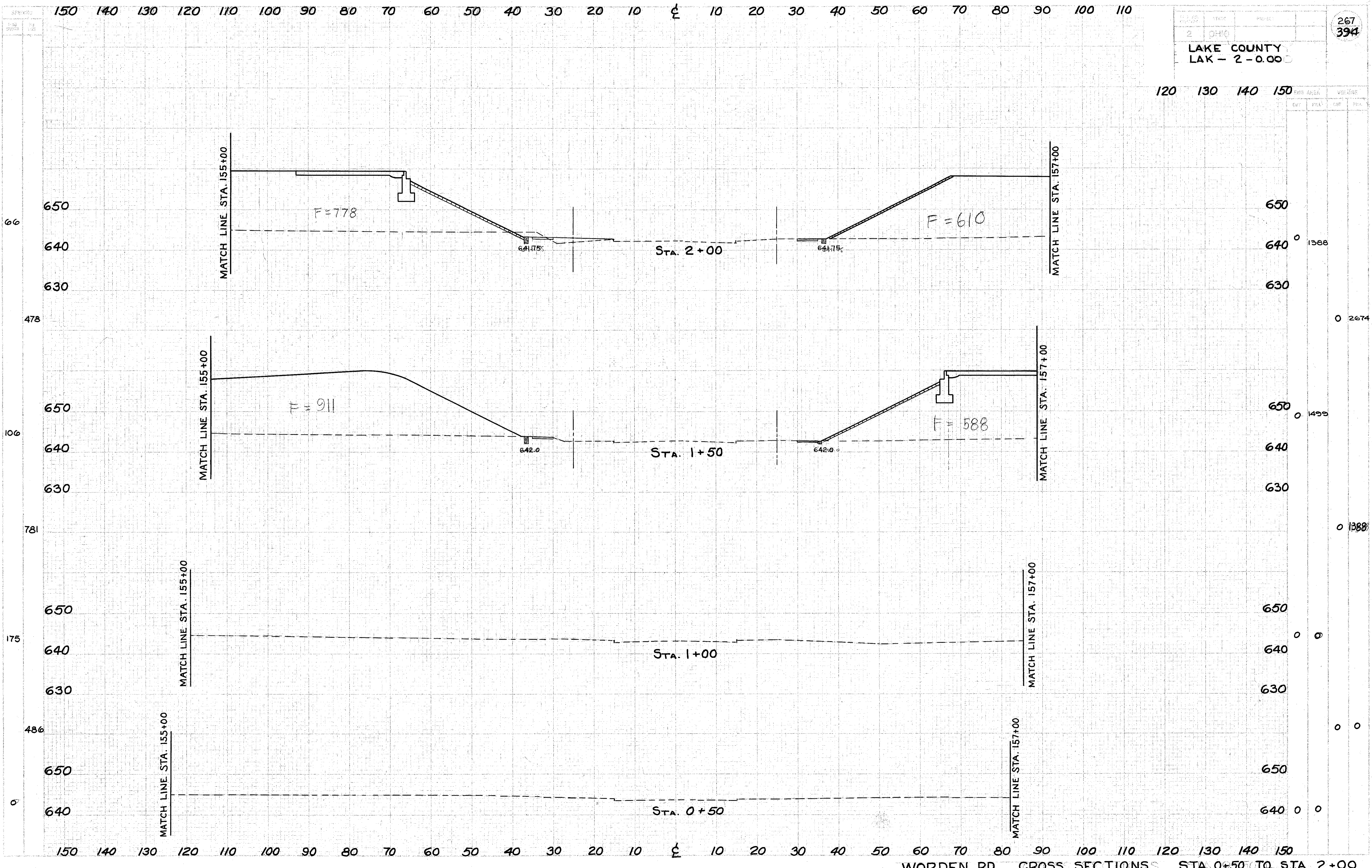
WORDEN RD. CROSS SECTIONS, STA. 0+50 TO STA. 2+00
