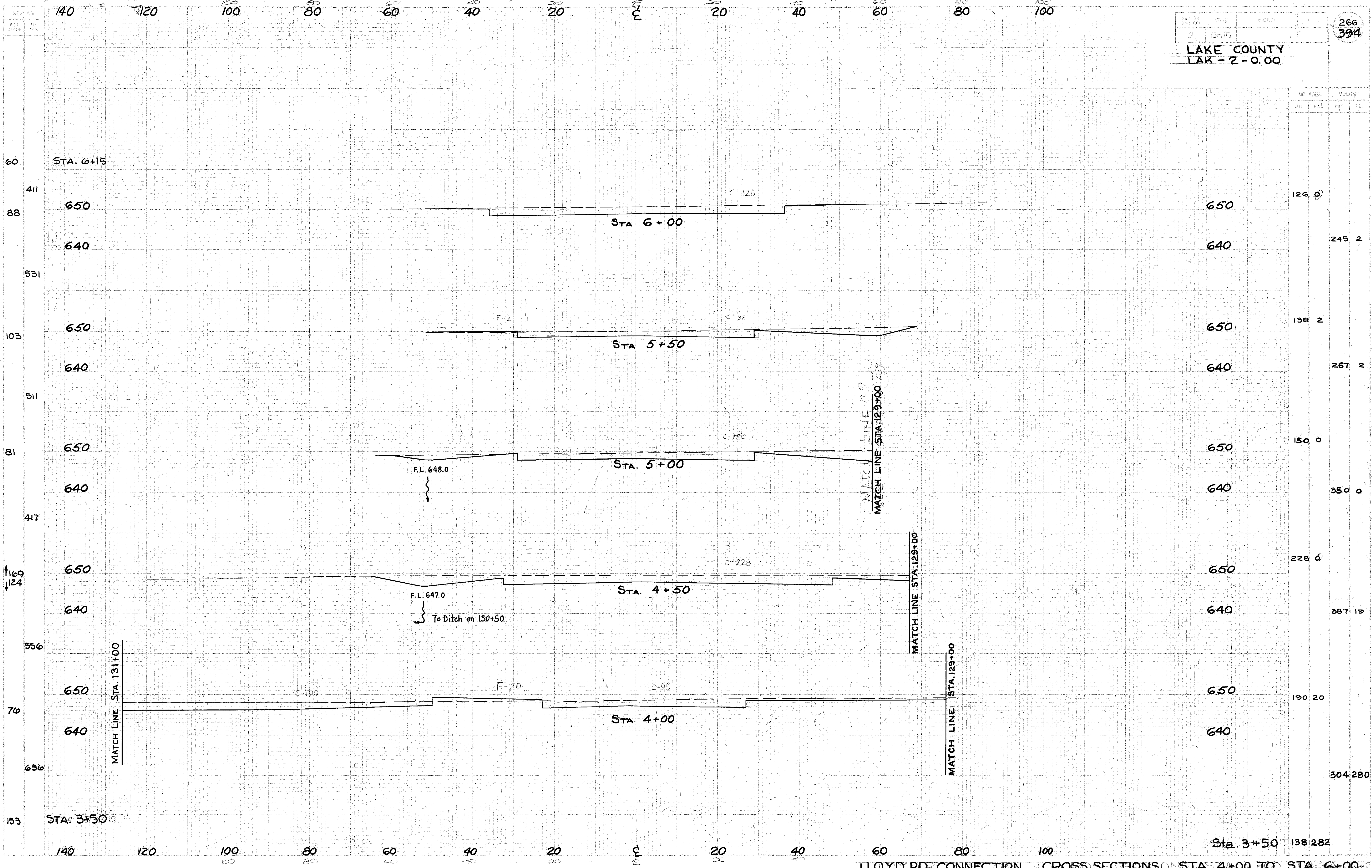
LLOYD RD CONNECTION CROSS SECTIONS ON STA 4+00 TO STA 6+00
