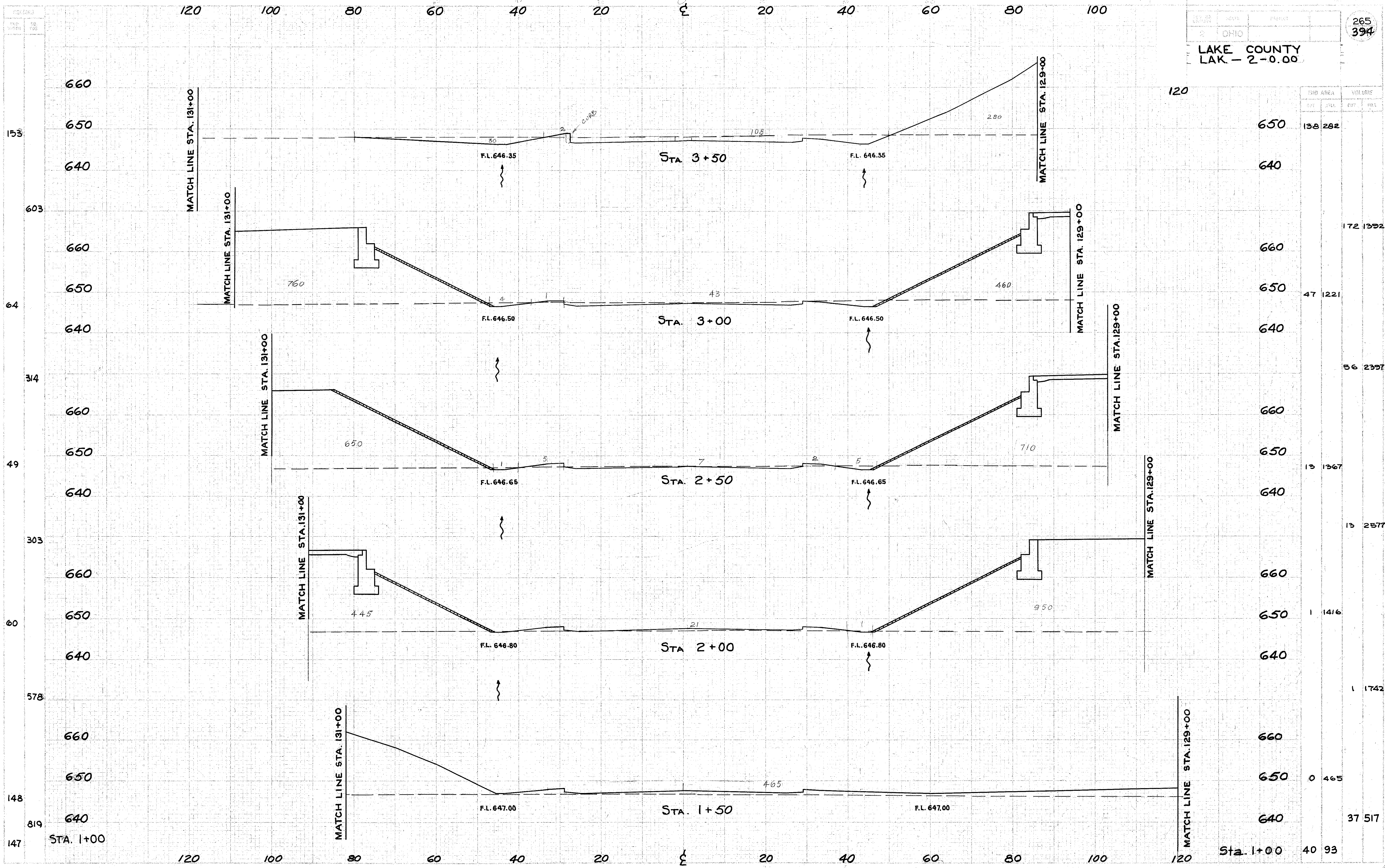
LLOYD RD. CONNECTION CROSS SECTIONS STA. 1+50 TO STA 3+50
