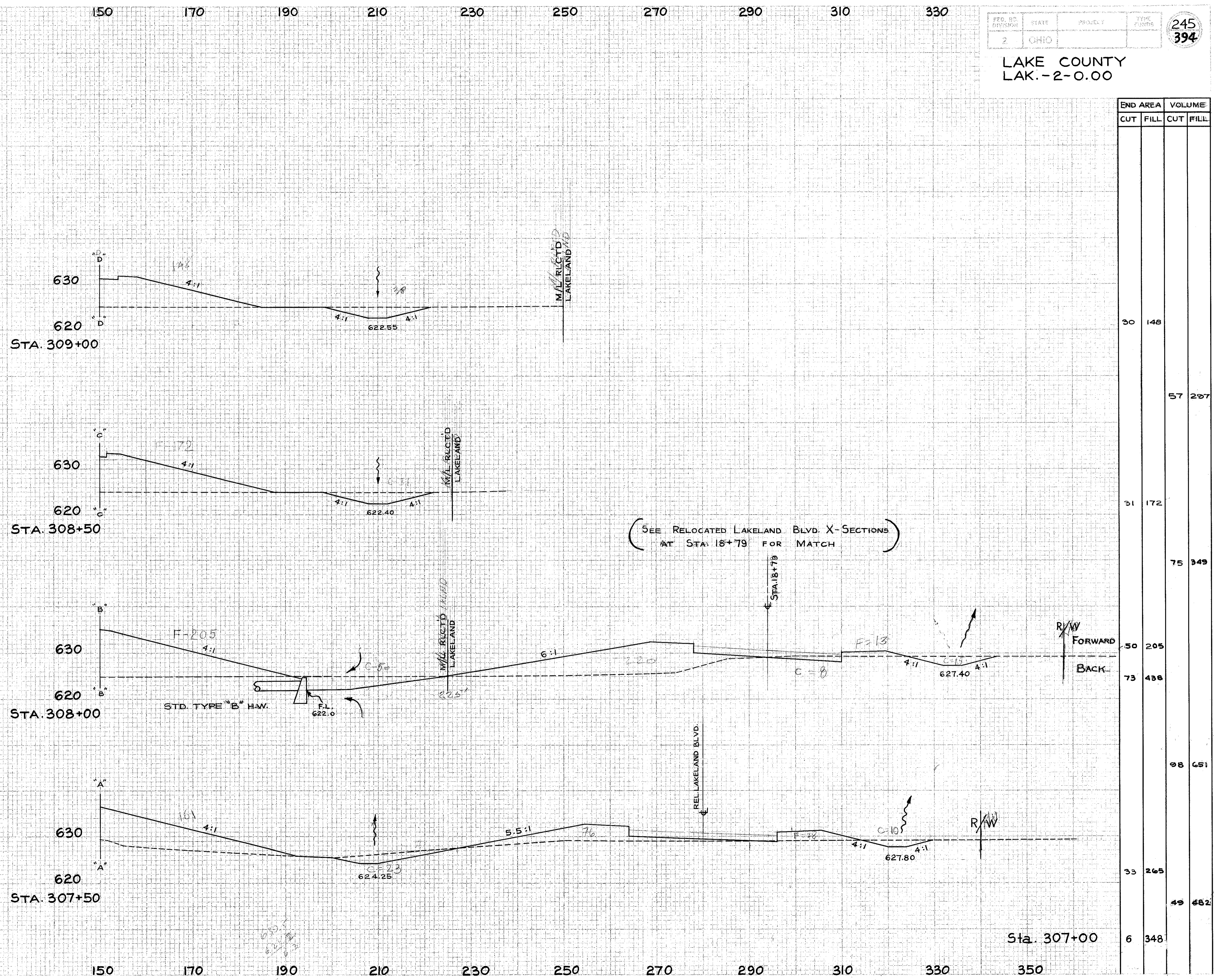
CROSS SECTIONS EXTENSIONS - STA. 307+50 TO STA. 309+00 - RIGHT
