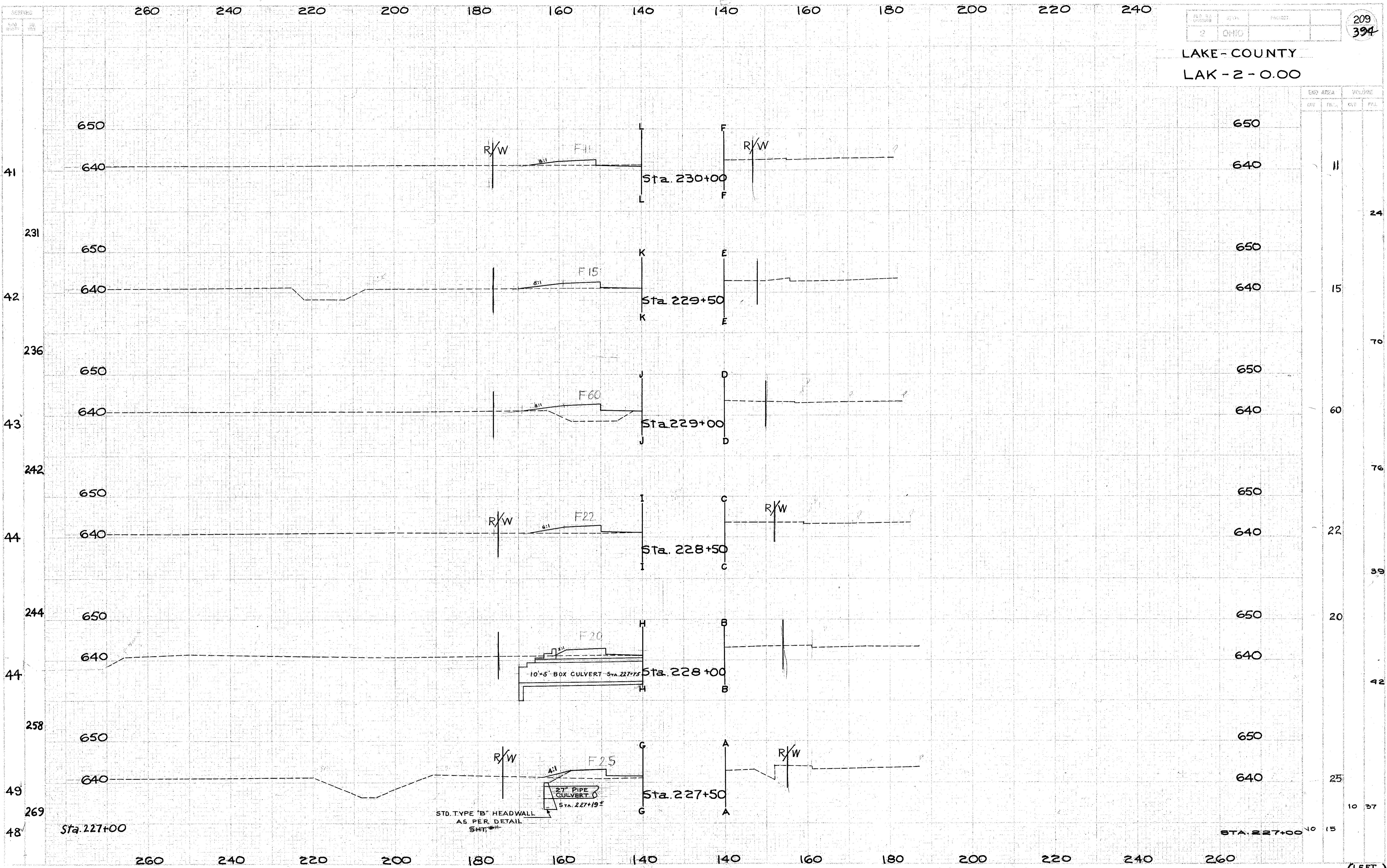
CROSS SECTION EXTENSIONS STA. 227+50 TO STA. 230+00 (LEFT RIGHT)
