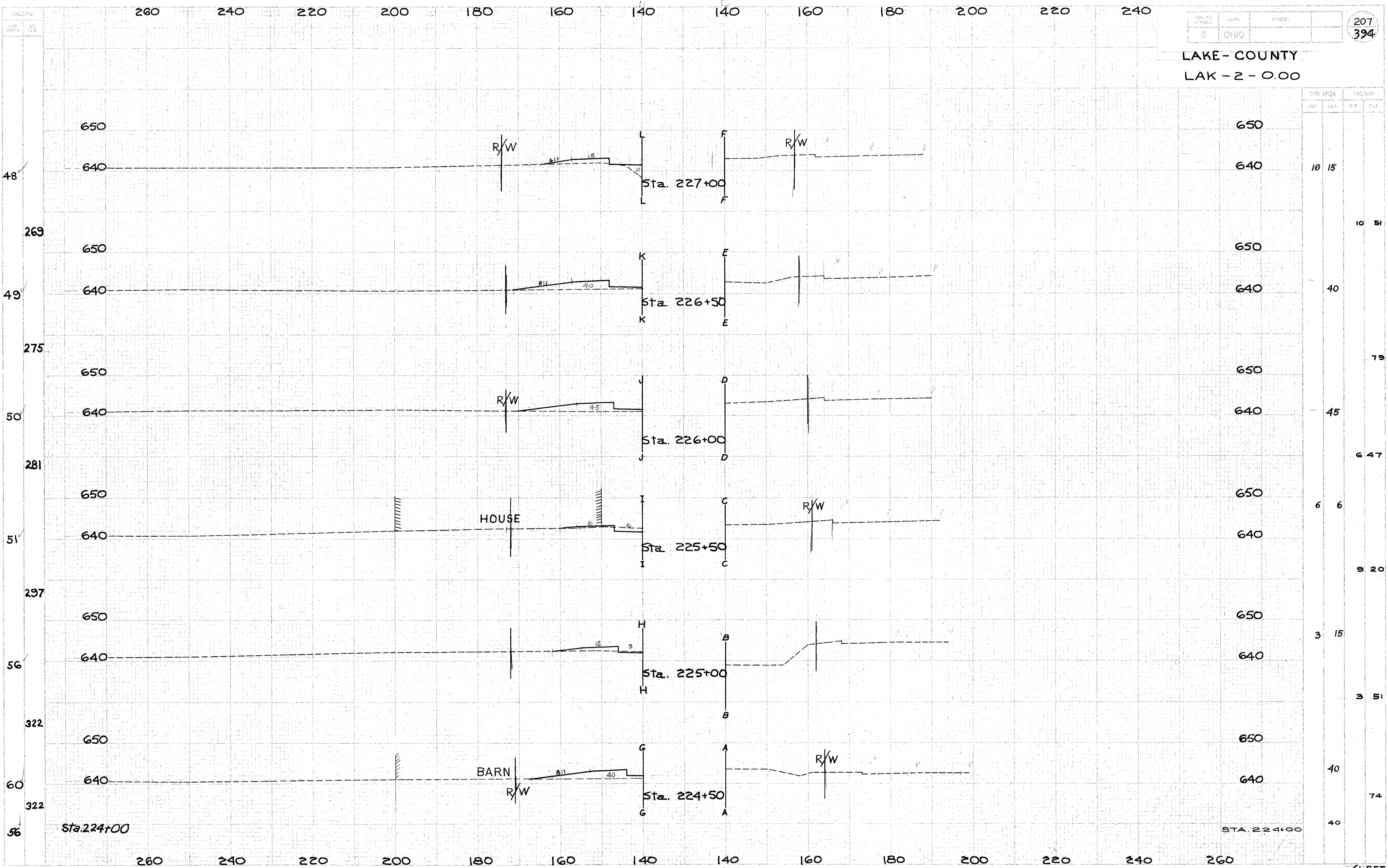
CROSS SECTION EXTENSIONS STA. 224+50 TO STA. 227+00 (LEFT RIGHT)
