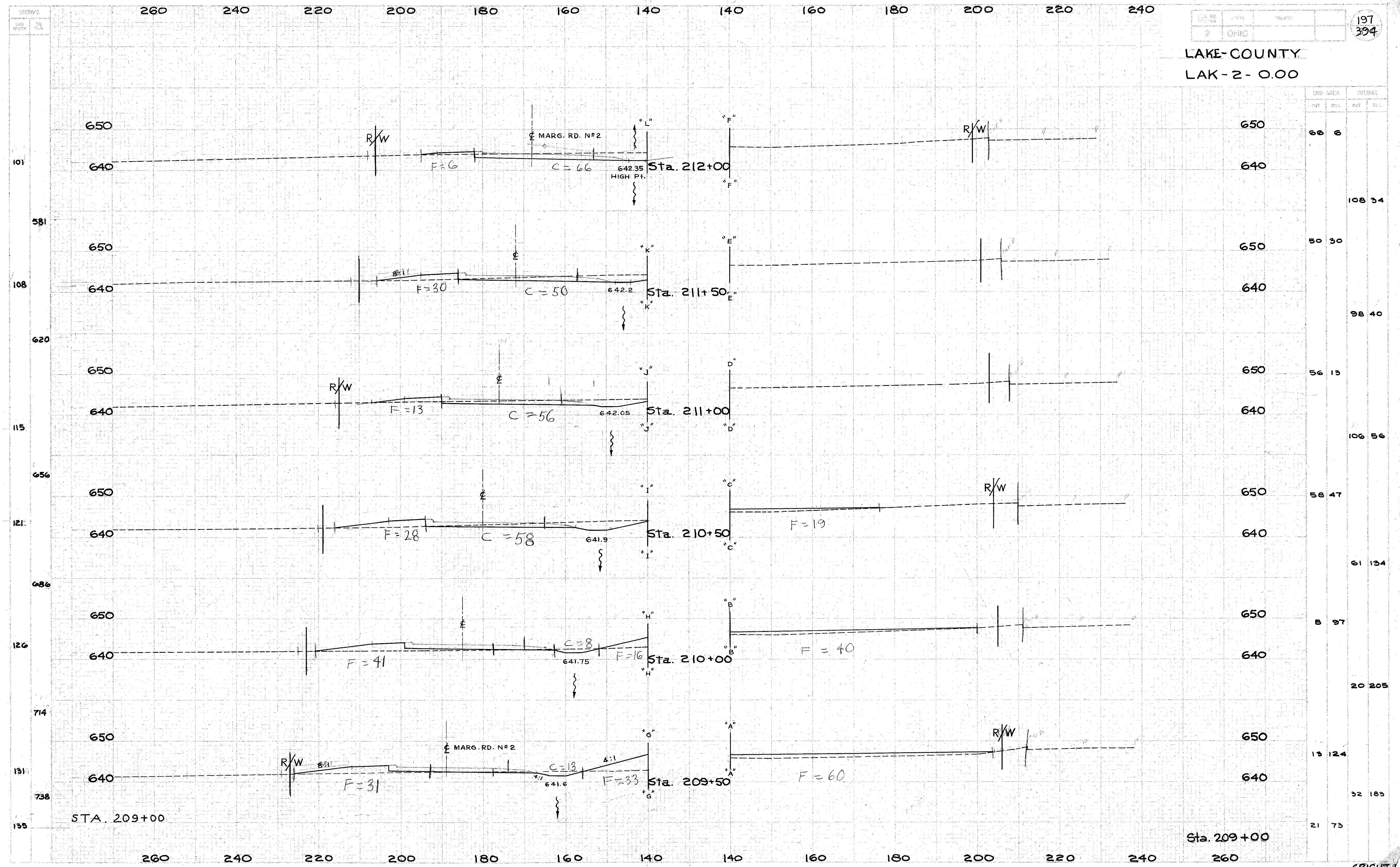
CROSS-SECTION EXTENSIONS STA. 209+50 TO STA. 212+00 (RIGHT LEFT)
