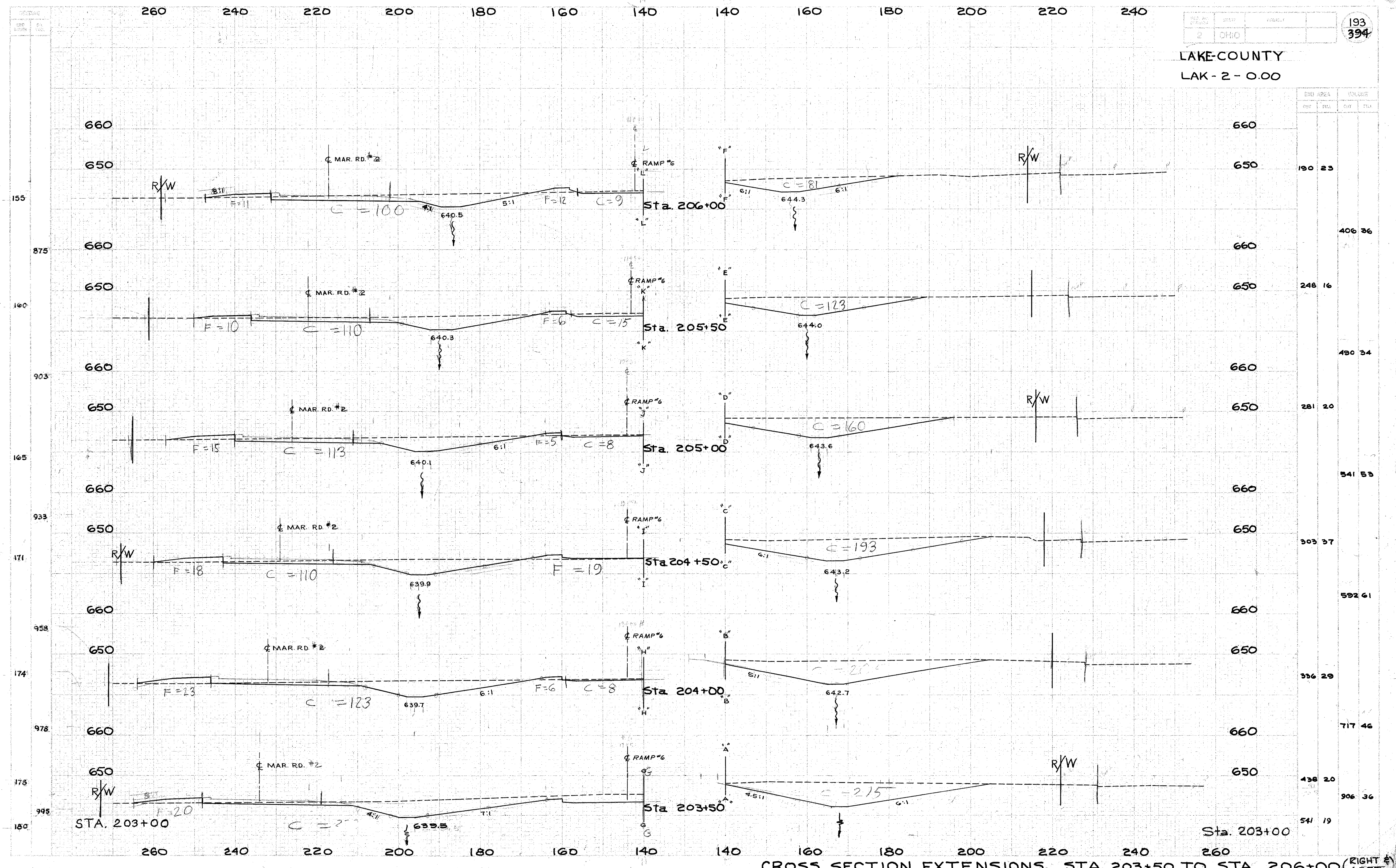
CROSS SECTION EXTENSIONS STA. 203+50 TO STA. 206+00 (RIGHT & LEFT)
