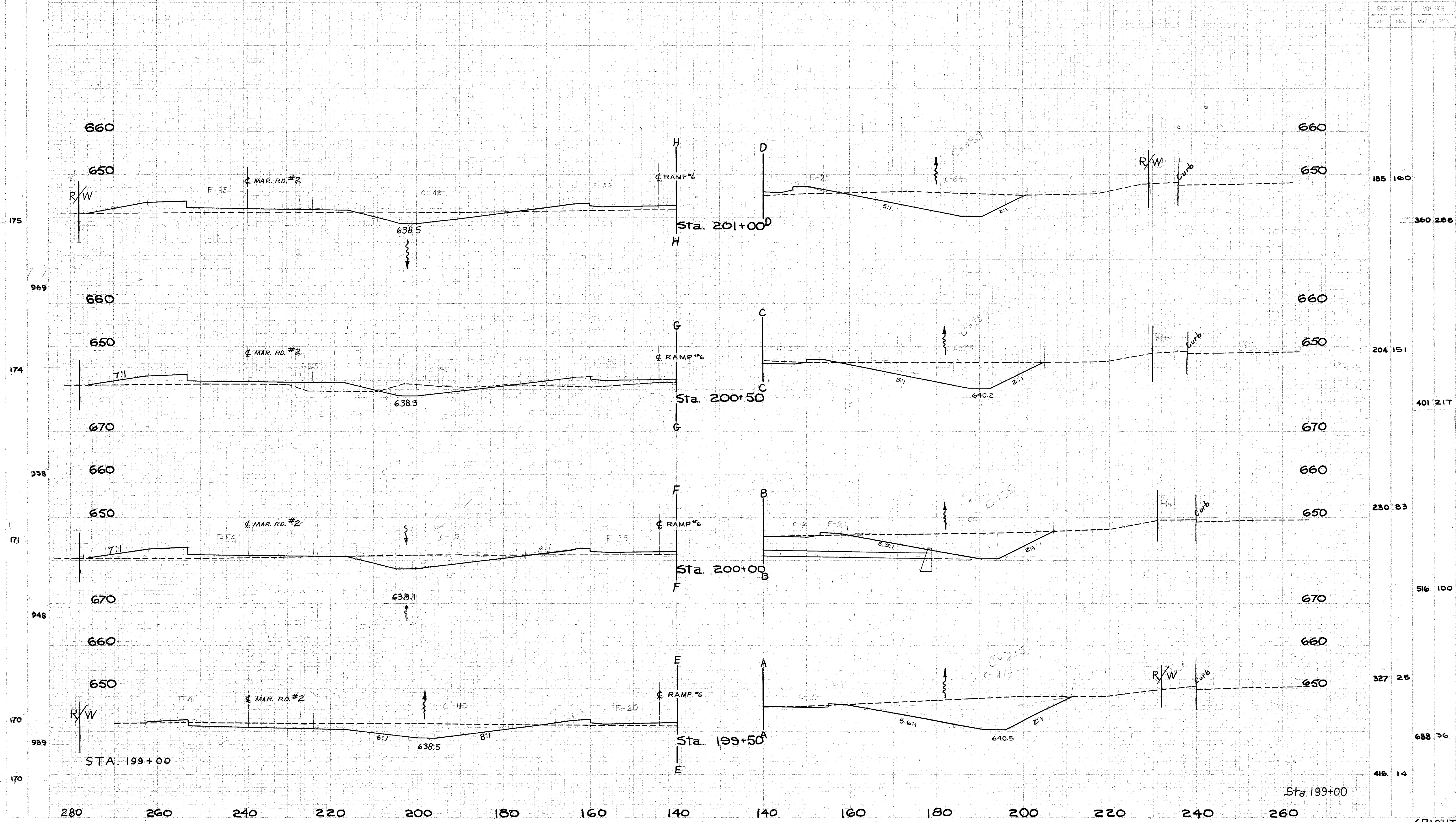
CROSS SECTION EXTENSIONS STA. 199+50 TO STA. 201+00 (RIGHT & LEFT)
