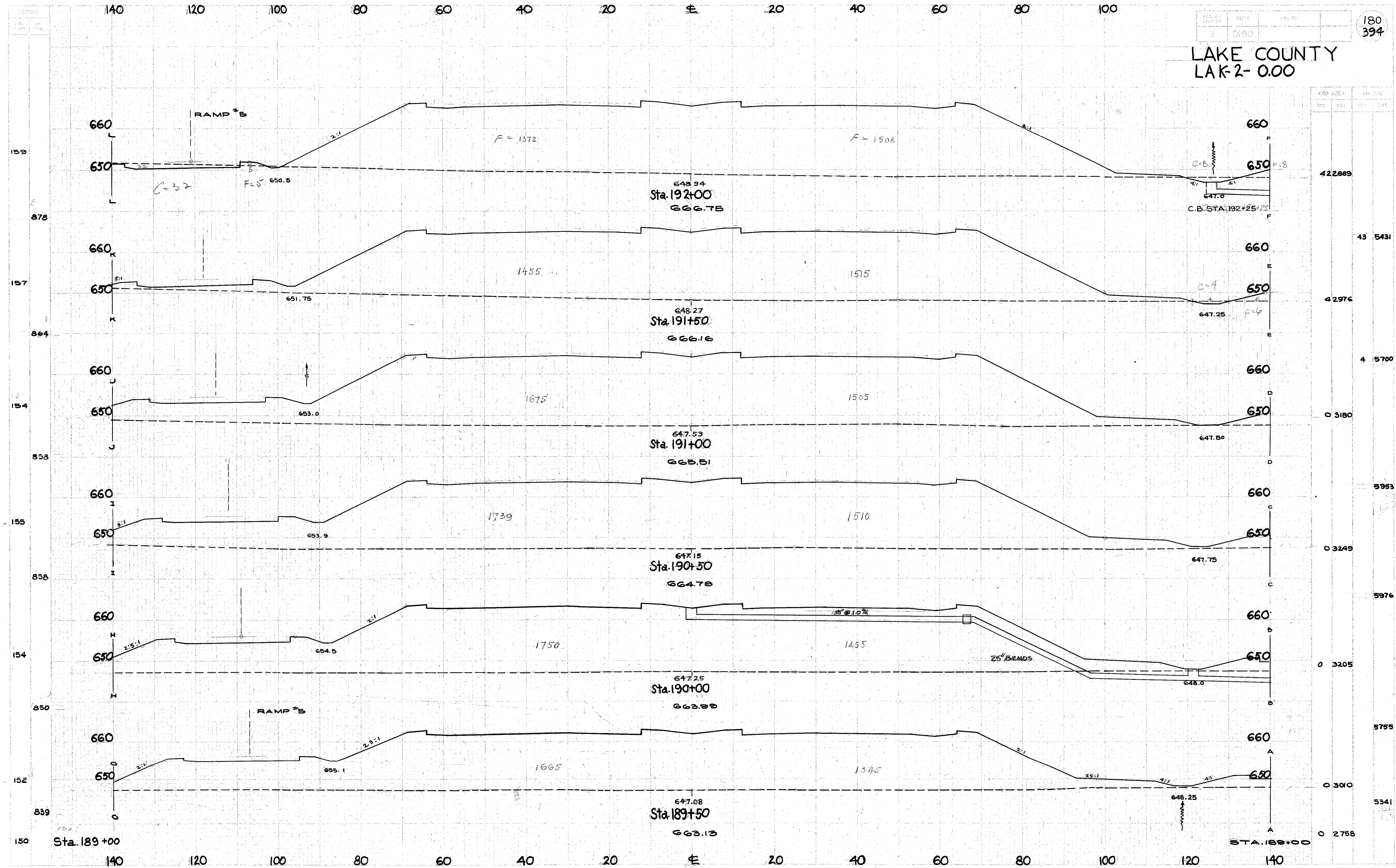
CROSS SECTIONS- STA.189+50 TO STA.192+00
